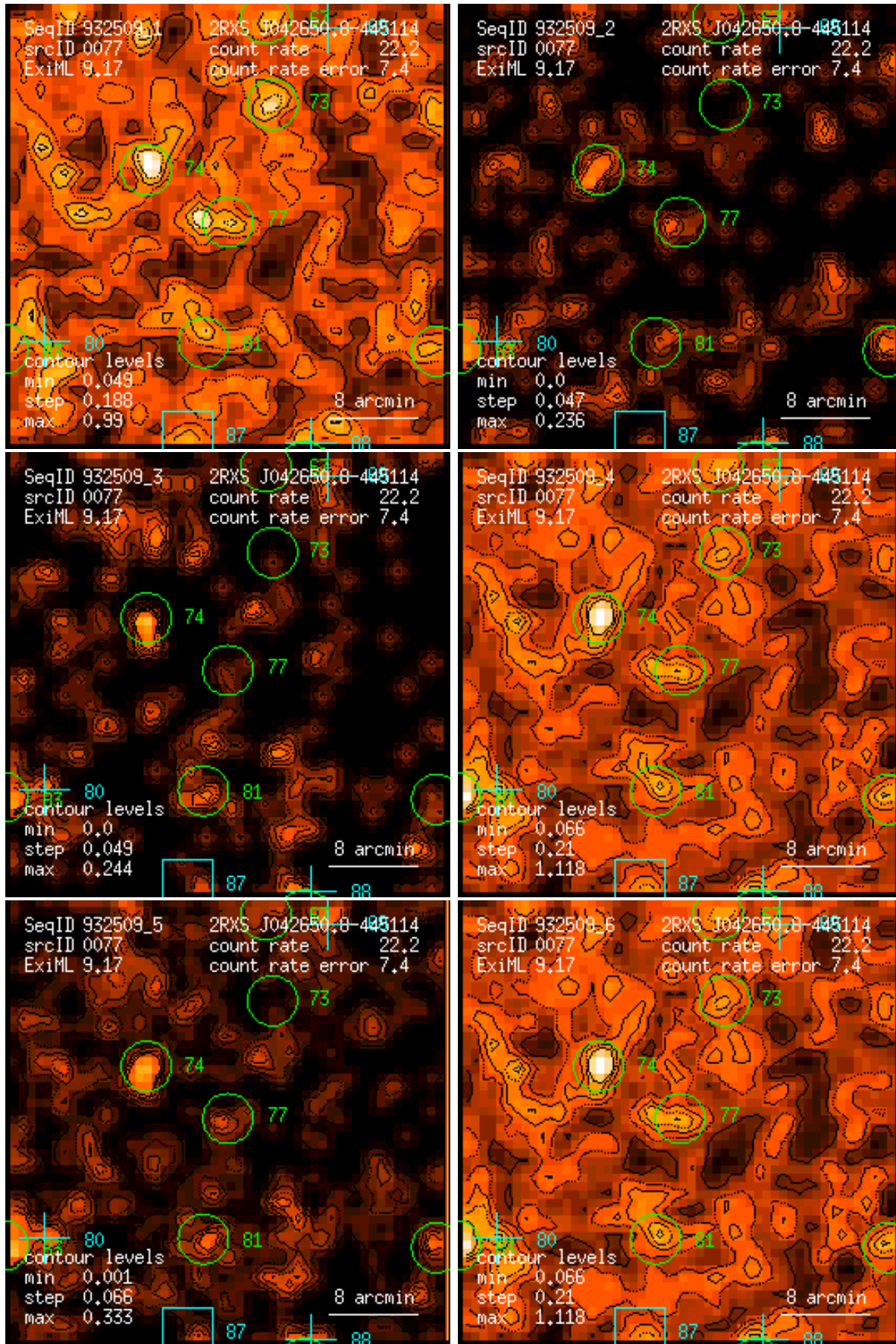
Figure 77: RASS 932509: detection 0077: band rate images, Gaussian filter: (1) PSPC channels 11 – 41, (2) 52 – 90, (3) 91 – 201, (4) 11 – 235, (5) 52 – 201, (6) 11 – 201. Broad band rates in counts/ks. Band rate contour levels in counts/ks/arcmin 2 .
