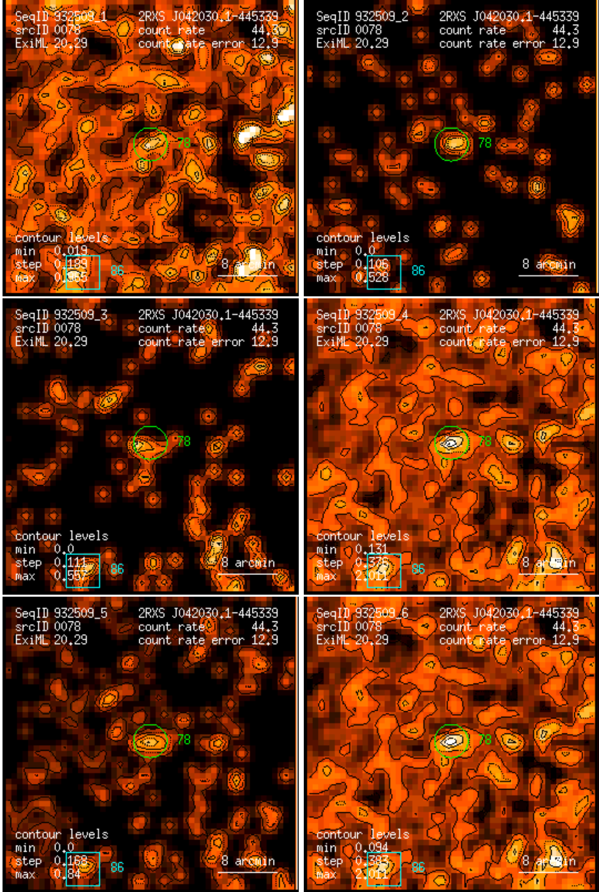
Figure 78: RASS 932509: detection 0078: band rate images, Gaussian filter: (1) PSPC channels 11 – 41, (2) 52 – 90, (3) 91 – 201, (4) 11 – 235, (5) 52 – 201, (6) 11 – 201. Broad band rates in counts/ks. Band rate contour levels in counts/ks/arcmin 2 .
