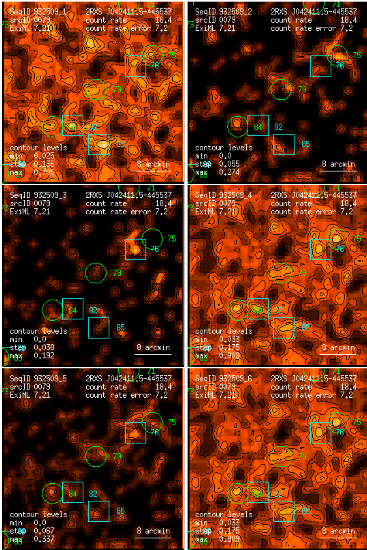
Figure 79: RASS 932509: detection 0079: band rate images, Gaussian filter: (1) PSPC channels 11 – 41, (2) 52 – 90, (3) 91 – 201, (4) 11 – 235, (5) 52 – 201, (6) 11 – 201. Broad band rates in counts/ks. Band rate contour levels in counts/ks/arcmin 2 .
