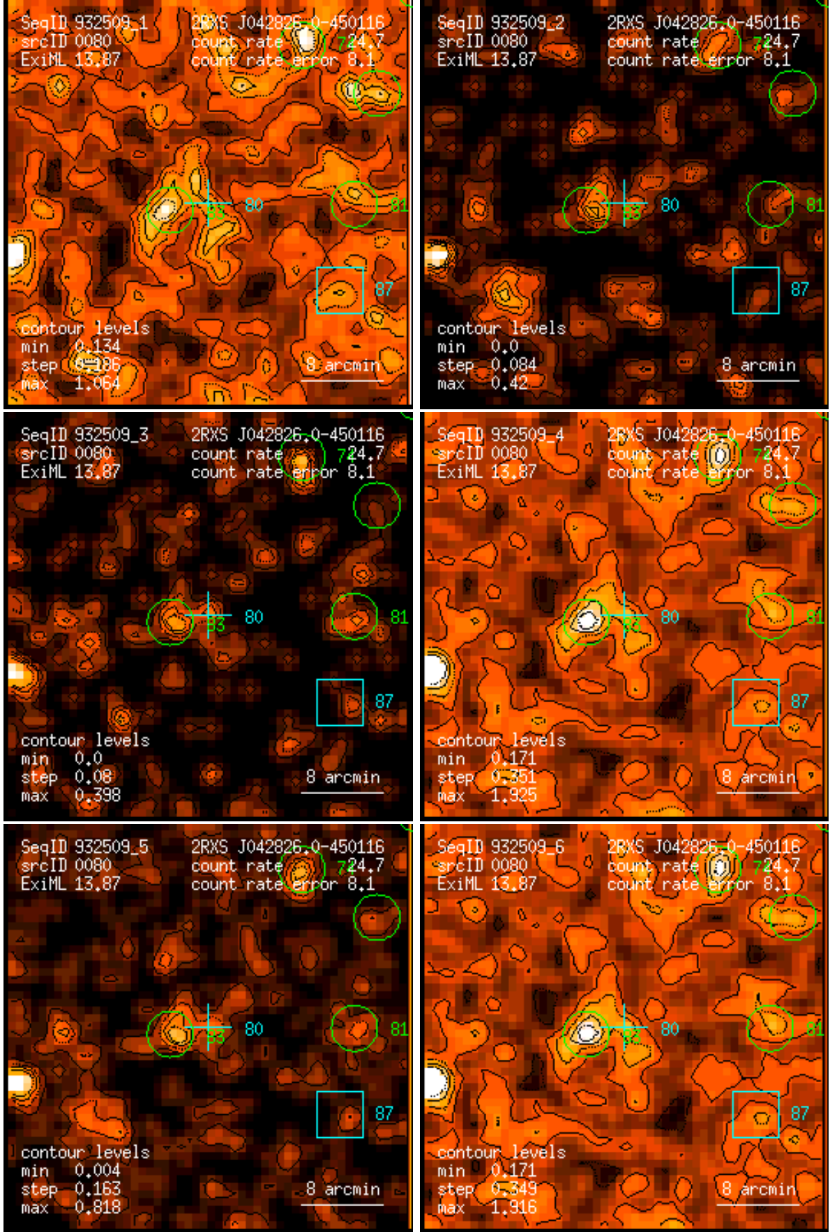
Figure 80: RASS 932509: detection 0080: band rate images, Gaussian filter: (1) PSPC channels 11 – 41, (2) 52 – 90, (3) 91 – 201, (4) 11 – 235, (5) 52 – 201, (6) 11 – 201. Broad band rates in counts/ks. Band rate contour levels in counts/ks/arcmin 2 .
