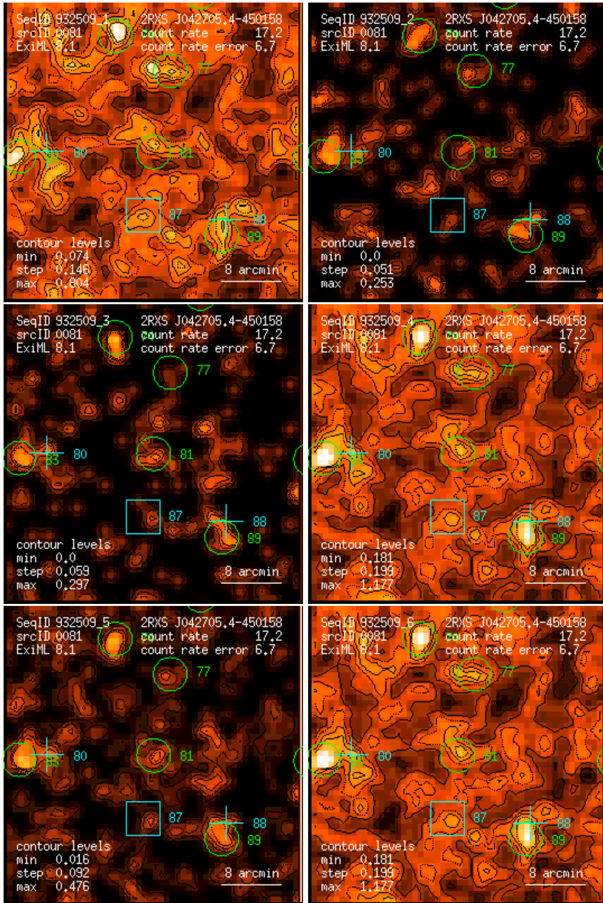
Figure 81: RASS 932509: detection 0081: band rate images, Gaussian filter: (1) PSPC channels 11 – 41, (2) 52 – 90, (3) 91 – 201, (4) 11 – 235, (5) 52 – 201, (6) 11 – 201. Broad band rates in counts/ks. Band rate contour levels in counts/ks/arcmin 2 .
