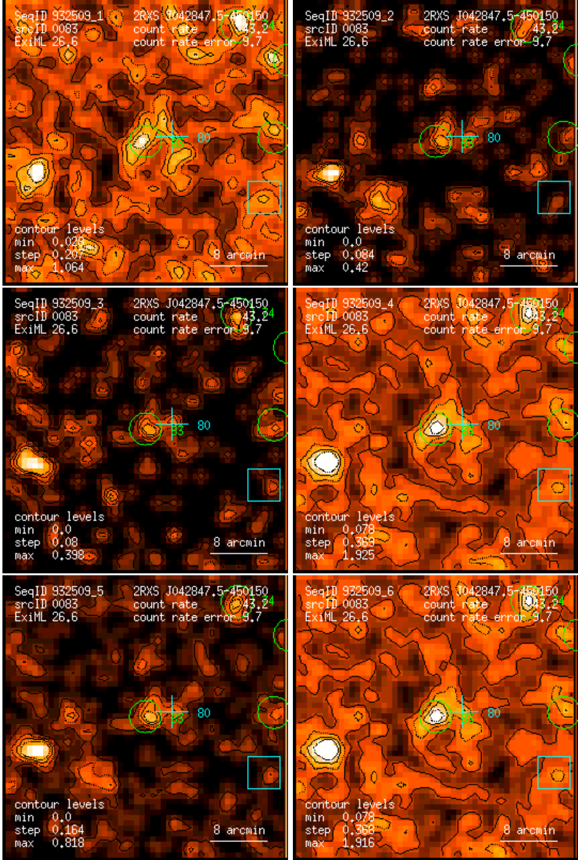
Figure 83: RASS 932509: detection 0083: band rate images, Gaussian filter: (1) PSPC channels 11 – 41, (2) 52 – 90, (3) 91 – 201, (4) 11 – 235, (5) 52 – 201, (6) 11 – 201. Broad band rates in counts/ks. Band rate contour levels in counts/ks/arcmin 2 .
