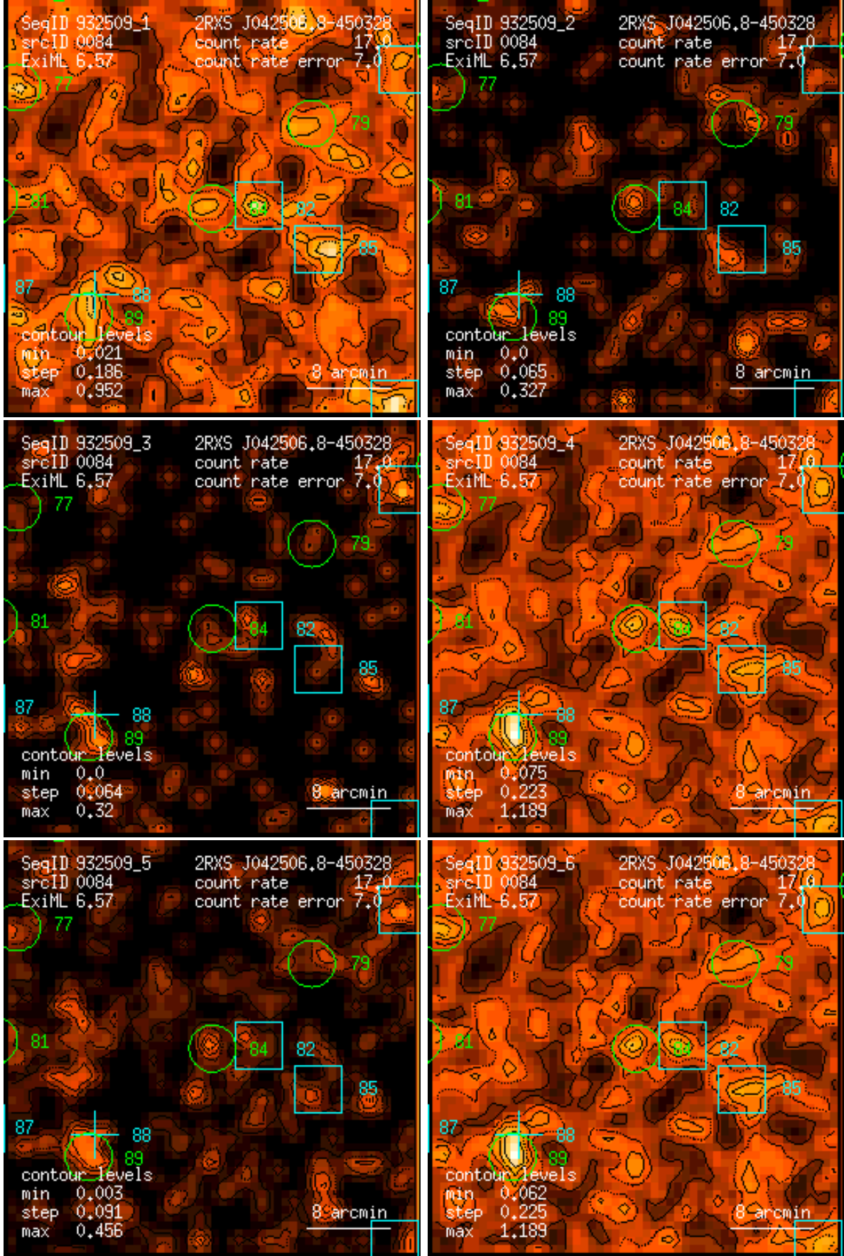
Figure 84: RASS 932509: detection 0084: band rate images, Gaussian filter: (1) PSPC channels 11 – 41, (2) 52 – 90, (3) 91 – 201, (4) 11 – 235, (5) 52 – 201, (6) 11 – 201. Broad band rates in counts/ks. Band rate contour levels in counts/ks/arcmin 2 .
