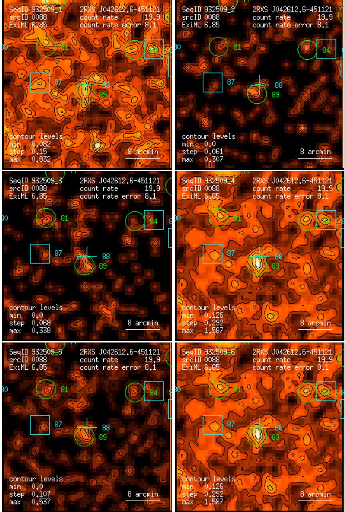
Figure 88: RASS 932509: detection 0088: band rate images, Gaussian filter: (1) PSPC channels 11 – 41, (2) 52 – 90, (3) 91 – 201, (4) 11 – 235, (5) 52 – 201, (6) 11 – 201. Broad band rates in counts/ks. Band rate contour levels in counts/ks/arcmin 2 .
