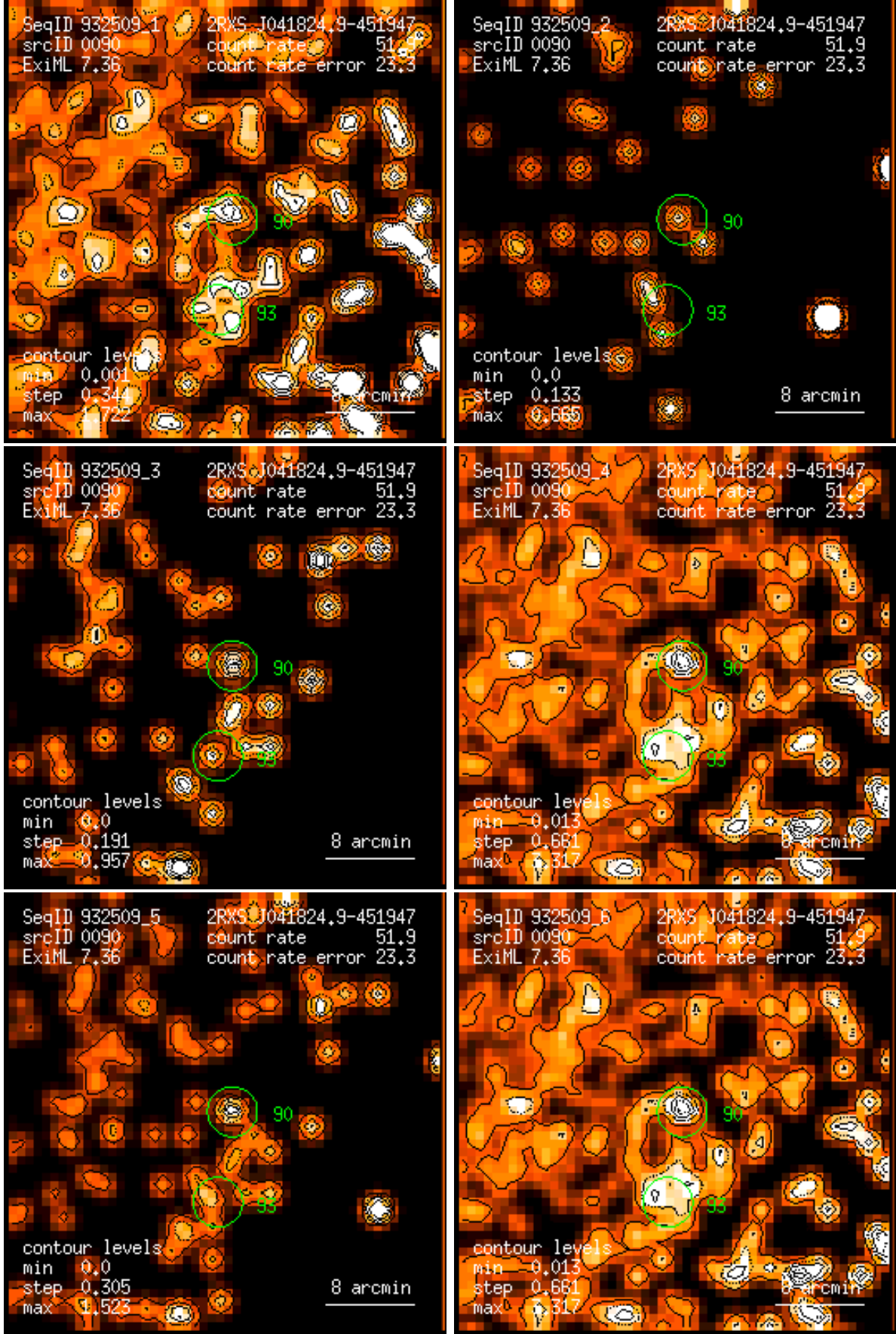
Figure 90: RASS 932509: detection 0090: band rate images, Gaussian filter: (1) PSPC channels 11 – 41, (2) 52 – 90, (3) 91 – 201, (4) 11 – 235, (5) 52 – 201, (6) 11 – 201. Broad band rates in counts/ks. Band rate contour levels in counts/ks/arcmin 2 .
