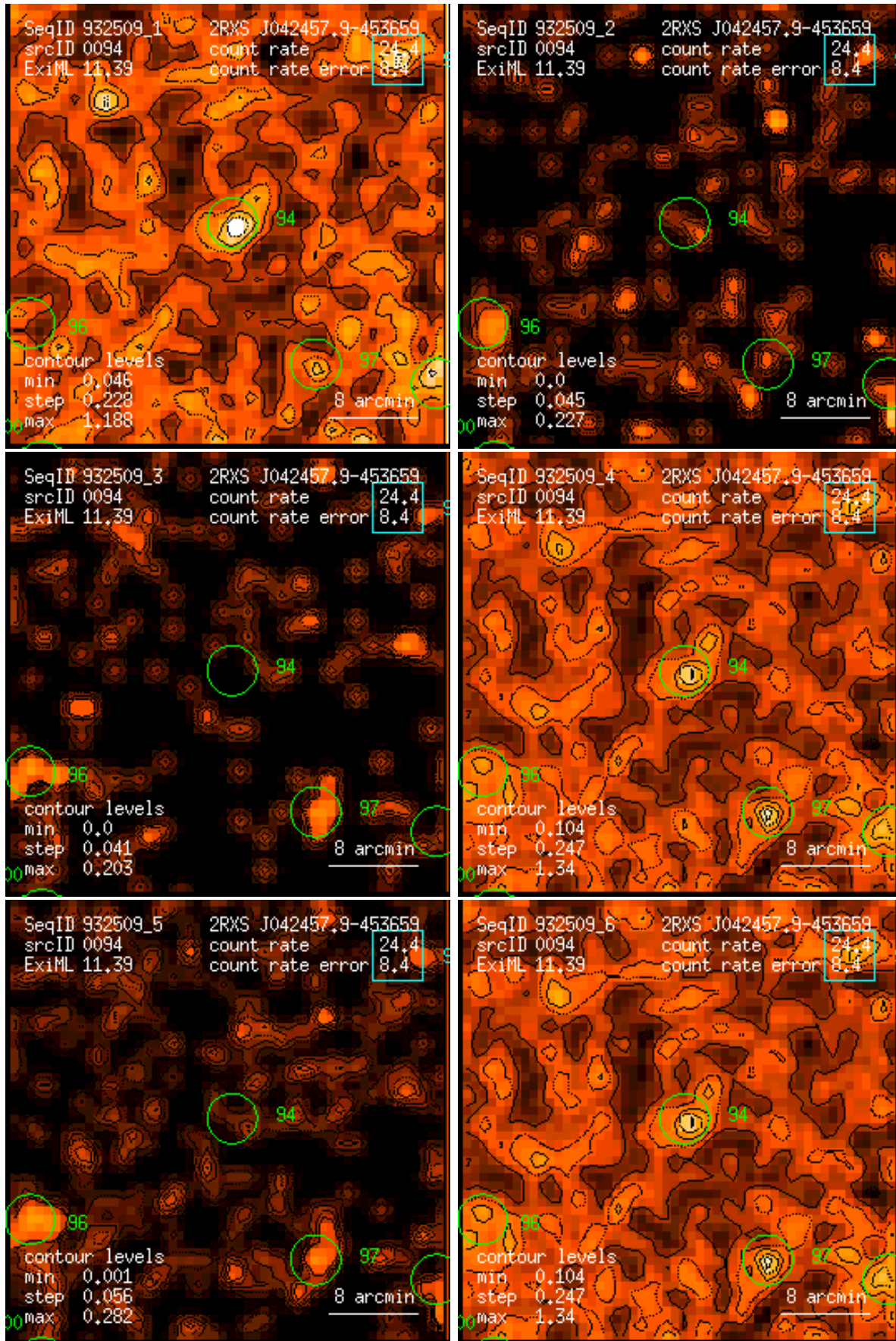
Figure 94: RASS 932509: detection 0094: band rate images, Gaussian filter: (1) PSPC channels 11 – 41, (2) 52 – 90, (3) 91 – 201, (4) 11 – 235, (5) 52 – 201, (6) 11 – 201. Broad band rates in counts/ks. Band rate contour levels in counts/ks/arcmin 2 .
