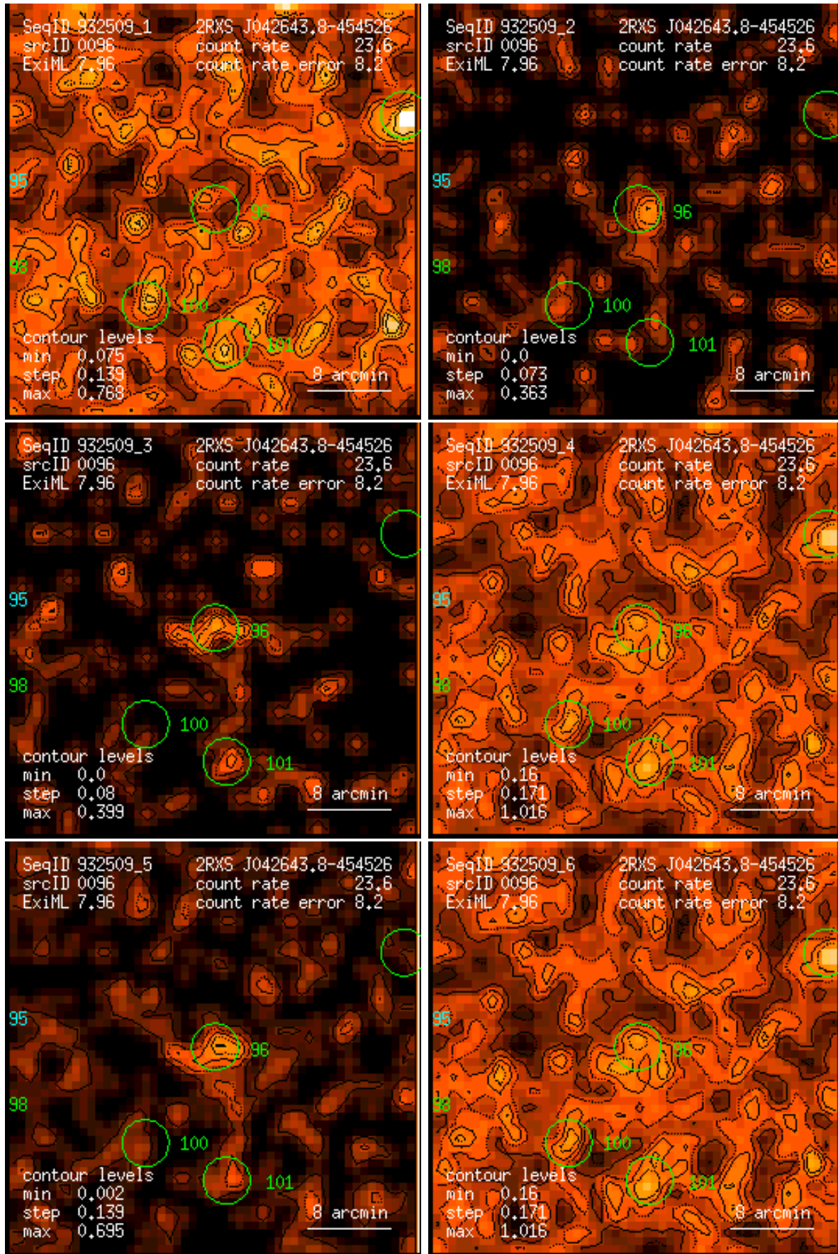
Figure 96: RASS 932509: detection 0096: band rate images, Gaussian filter: (1) PSPC channels 11 – 41, (2) 52 – 90, (3) 91 – 201, (4) 11 – 235, (5) 52 – 201, (6) 11 – 201. Broad band rates in counts/ks. Band rate contour levels in counts/ks/arcmin 2 .
