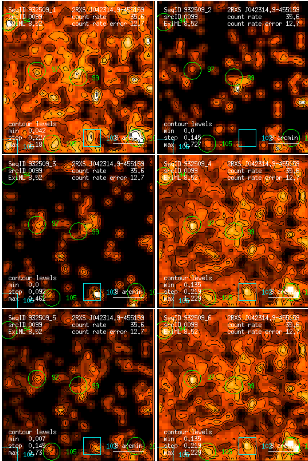
Figure 99: RASS 932509: detection 0099: band rate images, Gaussian filter: (1) PSPC channels 11 – 41, (2) 52 – 90, (3) 91 – 201, (4) 11 – 235, (5) 52 – 201, (6) 11 – 201. Broad band rates in counts/ks. Band rate contour levels in counts/ks/arcmin 2 .
