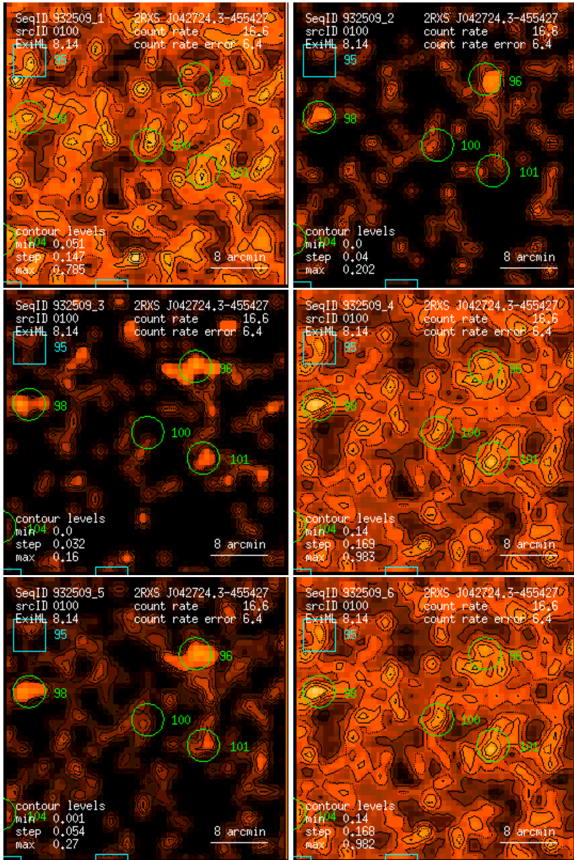
Figure 100: RASS 932509: detection 0100: band rate images, Gaussian filter: (1) PSPC channels 11 – 41, (2) 52 – 90, (3) 91 – 201, (4) 11 – 235, (5) 52 – 201, (6) 11 – 201. Broad band rates in counts/ks. Band rate contour levels in counts/ks/arcmin 2 .
