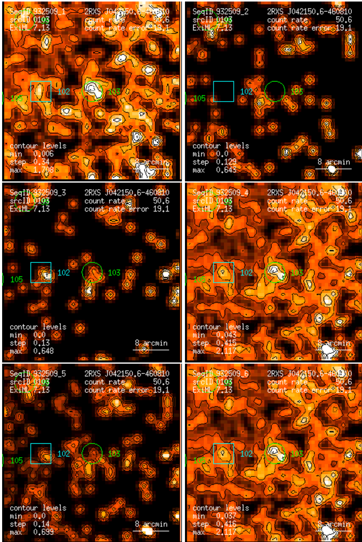
Figure 103: RASS 932509: detection 0103: band rate images, Gaussian filter: (1) PSPC channels 11 – 41, (2) 52 – 90, (3) 91 – 201, (4) 11 – 235, (5) 52 – 201, (6) 11 – 201. Broad band rates in counts/ks. Band rate contour levels in counts/ks/arcmin 2 .
