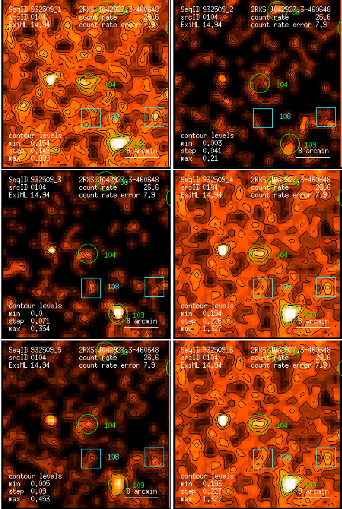
Figure 104: RASS 932509: detection 0104: band rate images, Gaussian filter: (1) PSPC channels 11 – 41, (2) 52 – 90, (3) 91 – 201, (4) 11 – 235, (5) 52 – 201, (6) 11 – 201. Broad band rates in counts/ks. Band rate contour levels in counts/ks/arcmin 2 .
