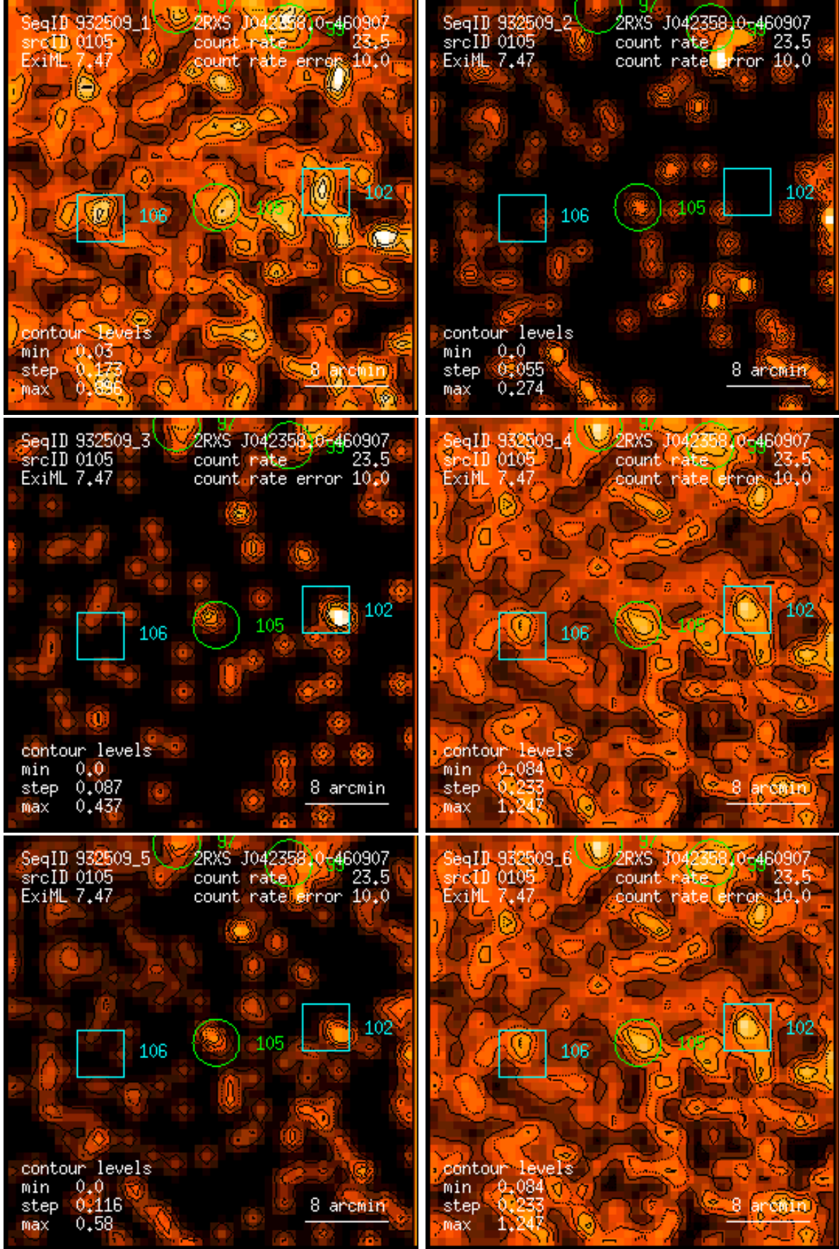
Figure 105: RASS 932509: detection 0105: band rate images, Gaussian filter: (1) PSPC channels 11 – 41, (2) 52 – 90, (3) 91 – 201, (4) 11 – 235, (5) 52 – 201, (6) 11 – 201. Broad band rates in counts/ks. Band rate contour levels in counts/ks/arcmin 2 .
