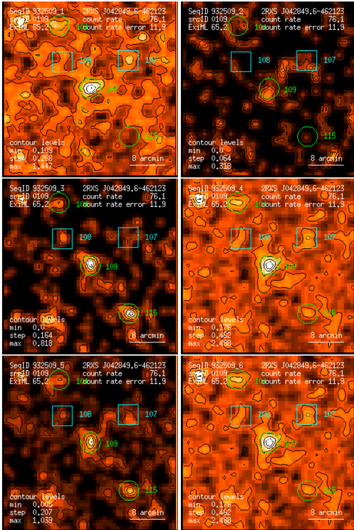
Figure 109: RASS 932509: detection 0109: band rate images, Gaussian filter: (1) PSPC channels 11 – 41, (2) 52 – 90, (3) 91 – 201, (4) 11 – 235, (5) 52 – 201, (6) 11 – 201. Broad band rates in counts/ks. Band rate contour levels in counts/ks/arcmin 2 .
