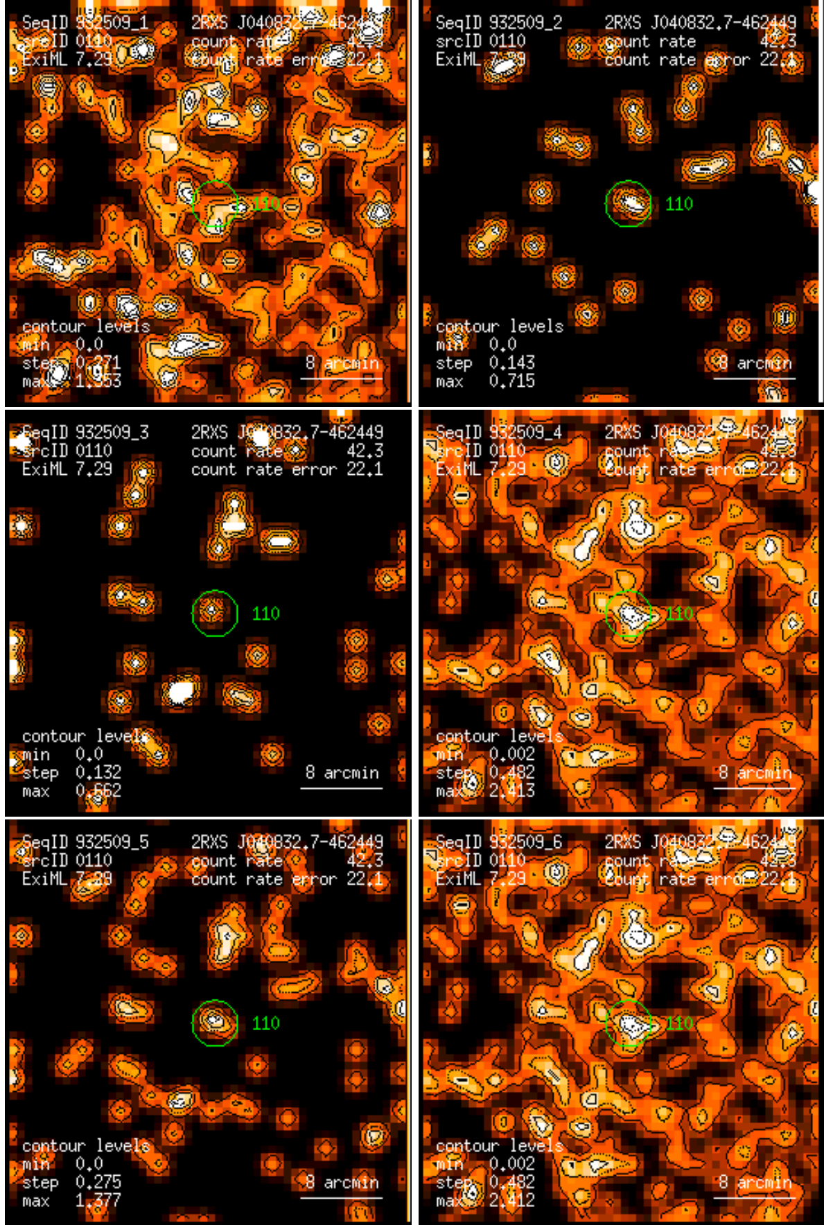
Figure 110: RASS 932509: detection 0110: band rate images, Gaussian filter: (1) PSPC channels 11 – 41, (2) 52 – 90, (3) 91 – 201, (4) 11 – 235, (5) 52 – 201, (6) 11 – 201. Broad band rates in counts/ks. Band rate contour levels in counts/ks/arcmin 2 .
