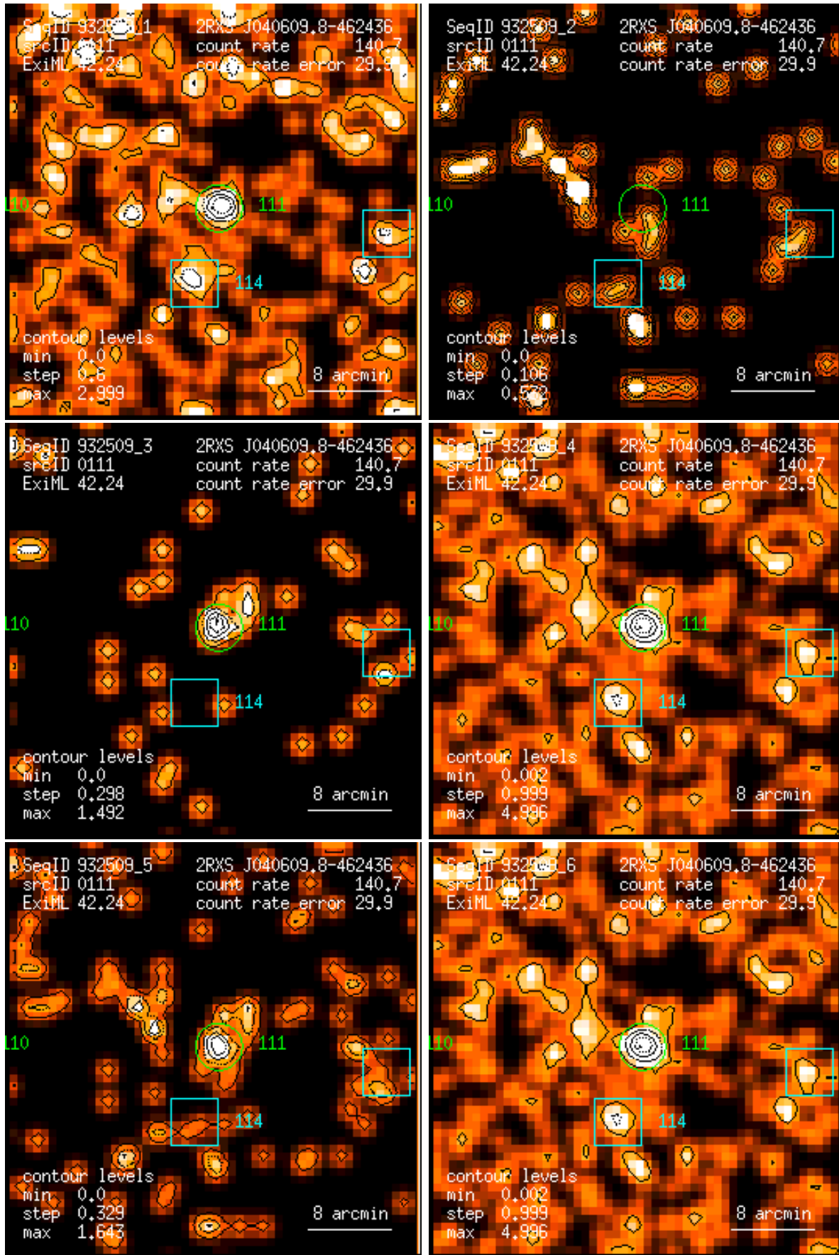
Figure 111: RASS 932509: detection 0111: band rate images, Gaussian filter: (1) PSPC channels 11 – 41, (2) 52 – 90, (3) 91 – 201, (4) 11 – 235, (5) 52 – 201, (6) 11 – 201. Broad band rates in counts/ks. Band rate contour levels in counts/ks/arcmin 2 .
