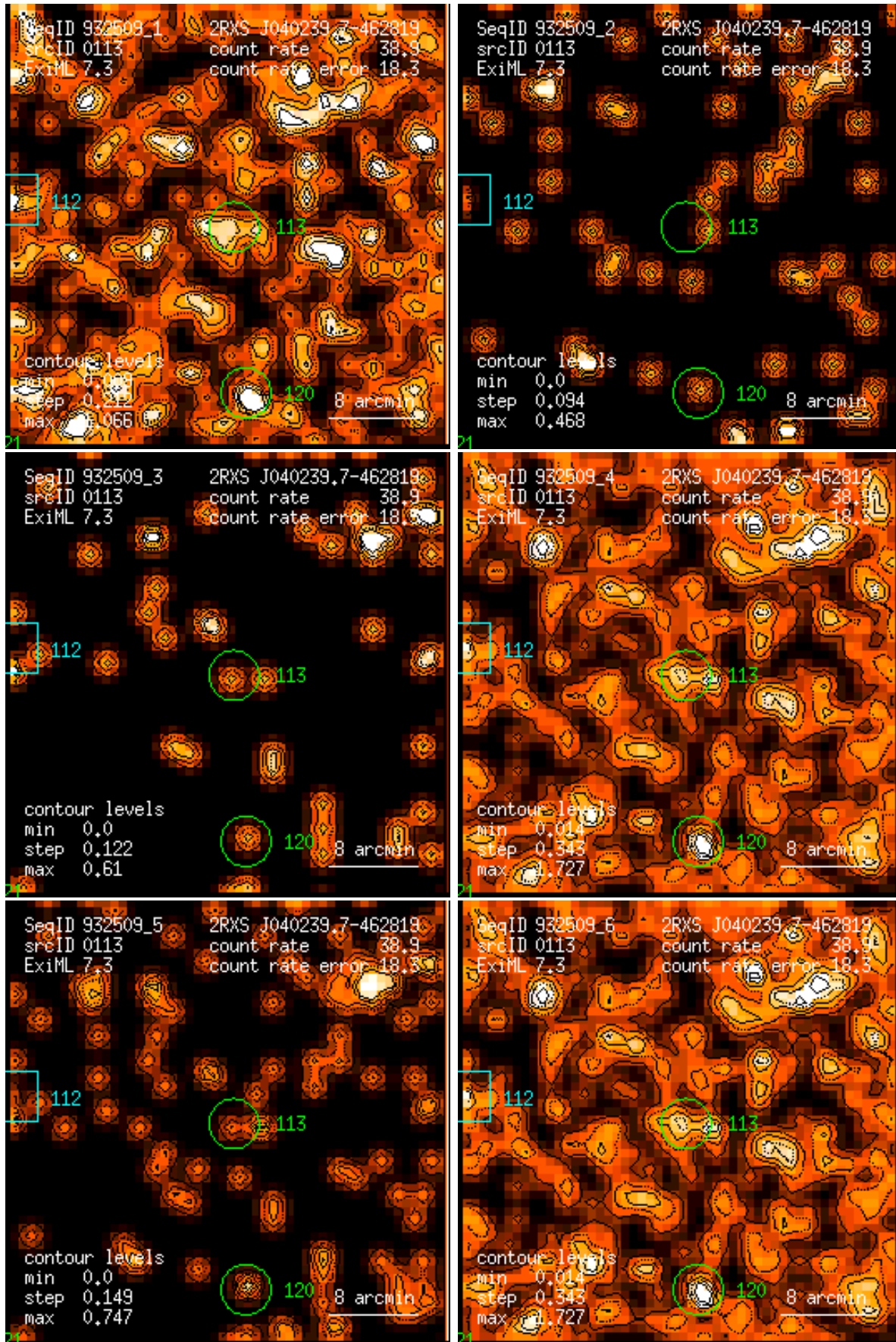
Figure 113: RASS 932509: detection 0113: band rate images, Gaussian filter: (1) PSPC channels 11 – 41, (2) 52 – 90, (3) 91 – 201, (4) 11 – 235, (5) 52 – 201, (6) 11 – 201. Broad band rates in counts/ks. Band rate contour levels in counts/ks/arcmin 2 .
