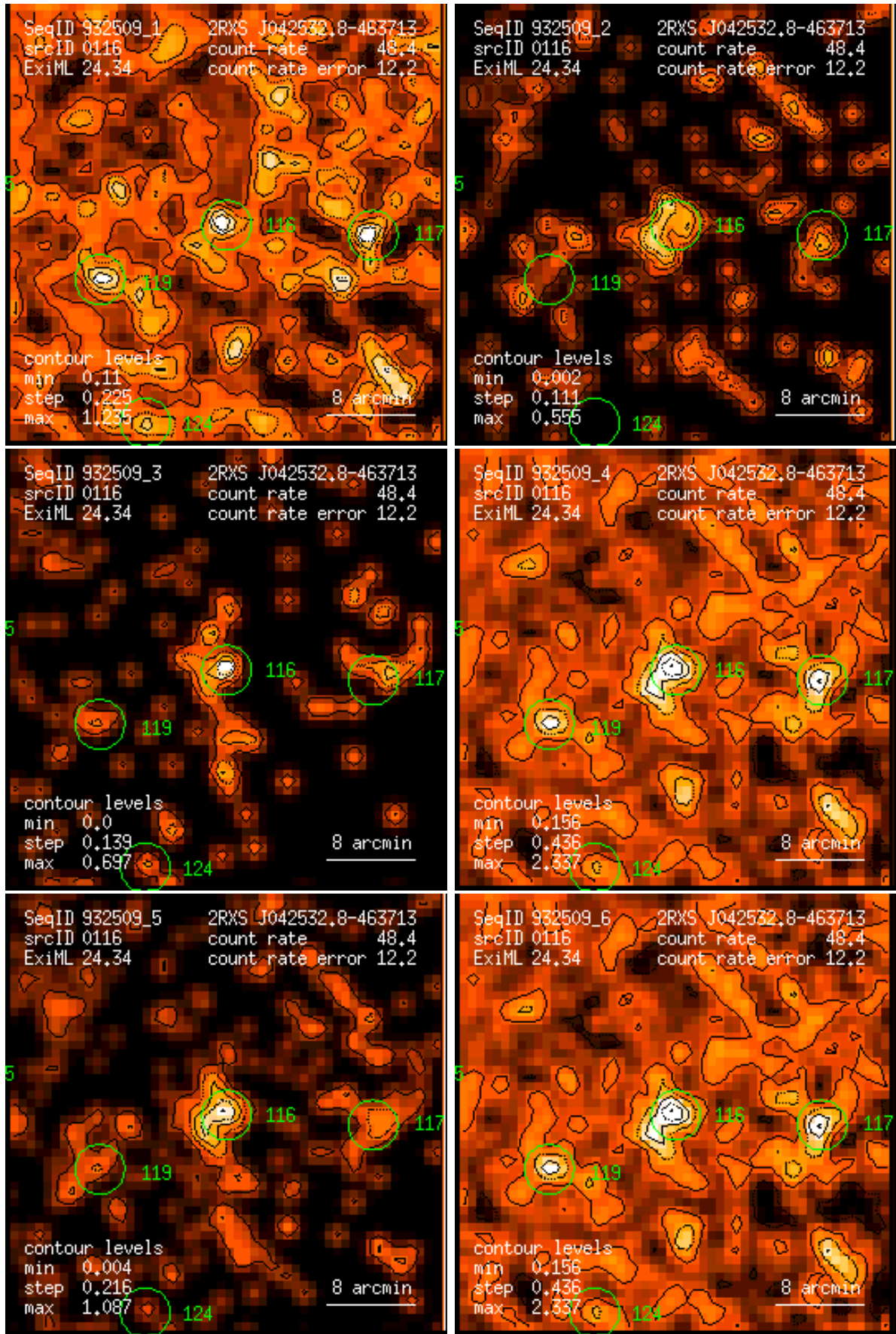
Figure 116: RASS 932509: detection 0116: band rate images, Gaussian filter: (1) PSPC channels 11 – 41, (2) 52 – 90, (3) 91 – 201, (4) 11 – 235, (5) 52 – 201, (6) 11 – 201. Broad band rates in counts/ks. Band rate contour levels in counts/ks/arcmin 2 .
