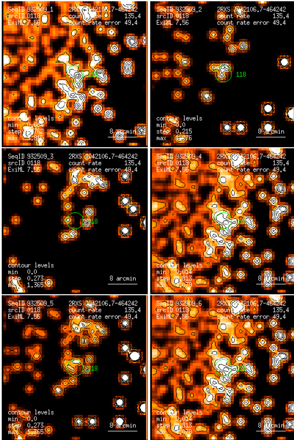
Figure 118: RASS 932509: detection 0118: band rate images, Gaussian filter: (1) PSPC channels 11 – 41, (2) 52 – 90, (3) 91 – 201, (4) 11 – 235, (5) 52 – 201, (6) 11 – 201. Broad band rates in counts/ks. Band rate contour levels in counts/ks/arcmin 2 .
