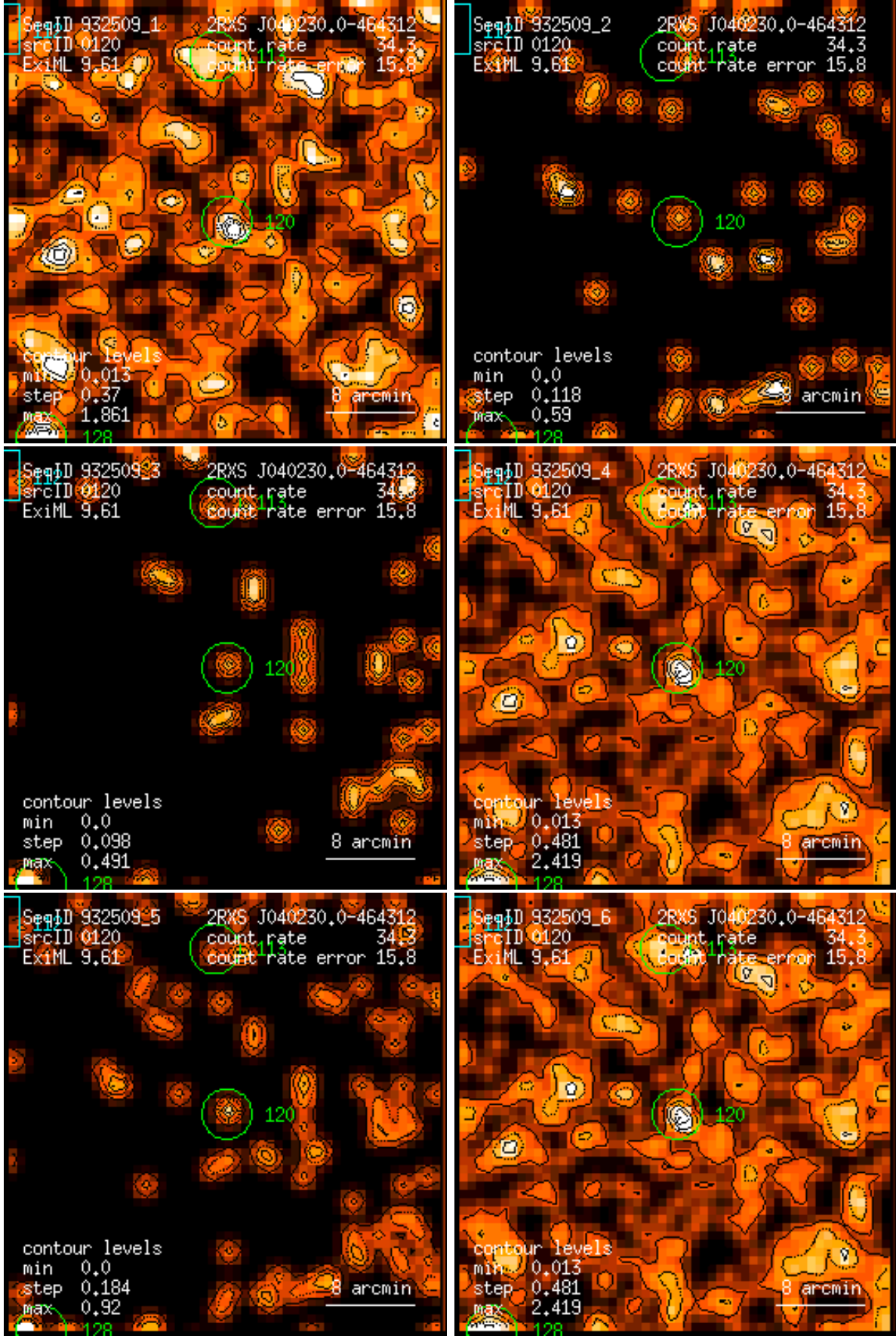
Figure 120: RASS 932509: detection 0120: band rate images, Gaussian filter: (1) PSPC channels 11 – 41, (2) 52 – 90, (3) 91 – 201, (4) 11 – 235, (5) 52 – 201, (6) 11 – 201. Broad band rates in counts/ks. Band rate contour levels in counts/ks/arcmin 2 .
