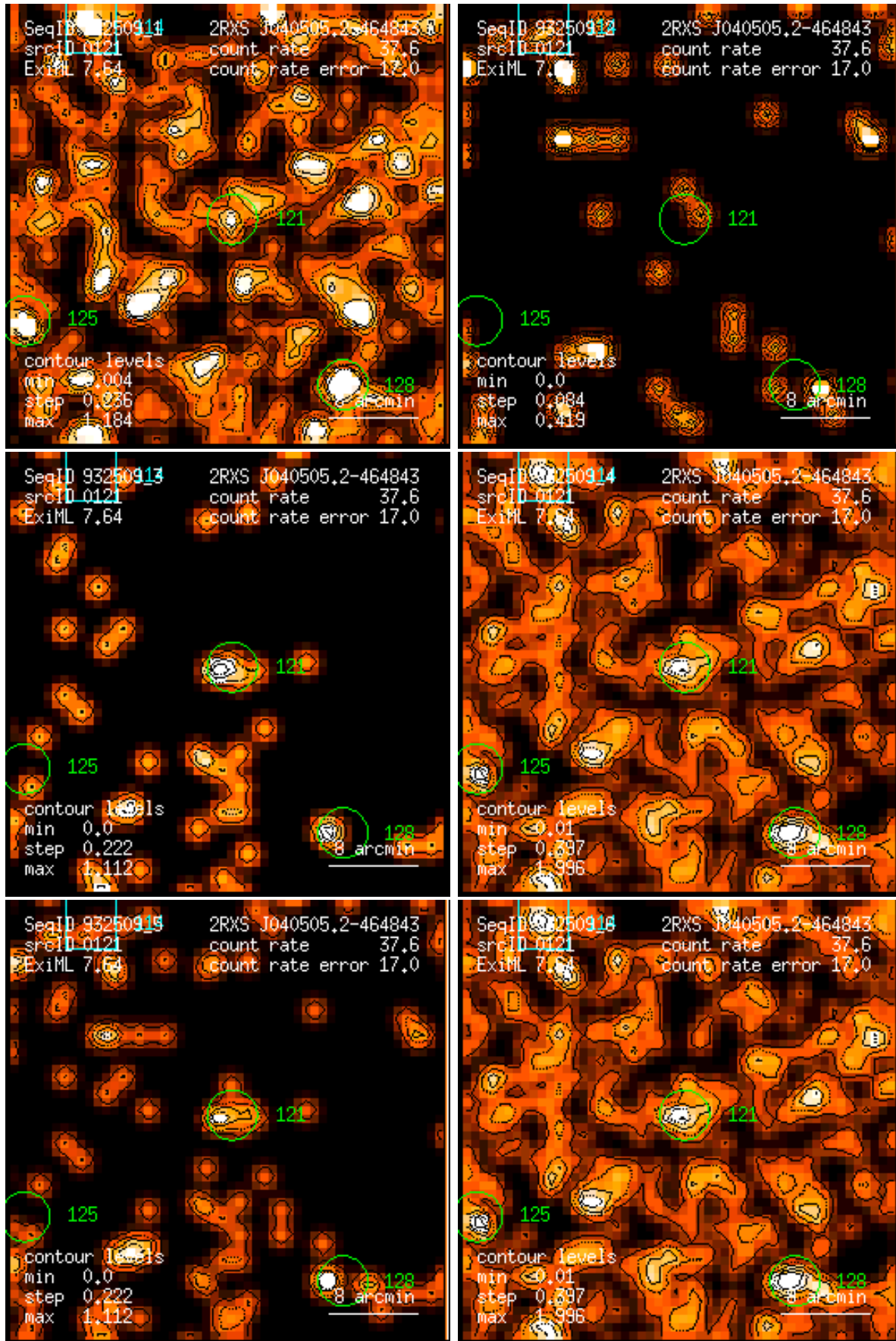
Figure 121: RASS 932509: detection 0121: band rate images, Gaussian filter: (1) PSPC channels 11 – 41, (2) 52 – 90, (3) 91 – 201, (4) 11 – 235, (5) 52 – 201, (6) 11 – 201. Broad band rates in counts/ks. Band rate contour levels in counts/ks/arcmin 2 .
