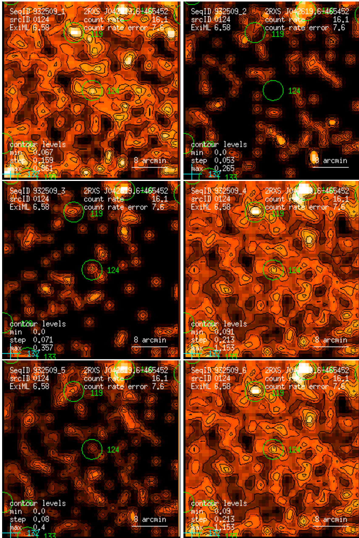
Figure 124: RASS 932509: detection 0124: band rate images, Gaussian filter: (1) PSPC channels 11 – 41, (2) 52 – 90, (3) 91 – 201, (4) 11 – 235, (5) 52 – 201, (6) 11 – 201. Broad band rates in counts/ks. Band rate contour levels in counts/ks/arcmin 2 .
