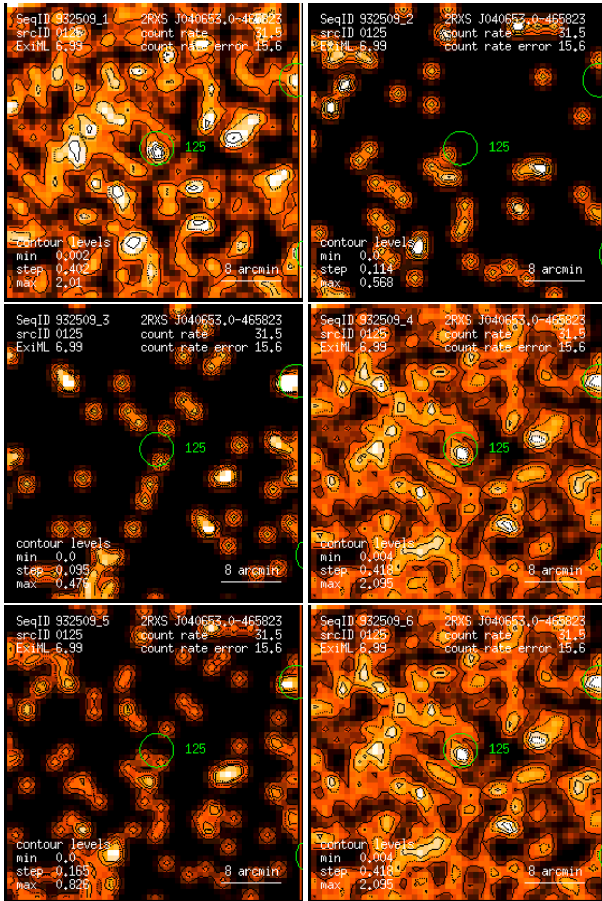
Figure 125: RASS 932509: detection 0125: band rate images, Gaussian filter: (1) PSPC channels 11 – 41, (2) 52 – 90, (3) 91 – 201, (4) 11 – 235, (5) 52 – 201, (6) 11 – 201. Broad band rates in counts/ks. Band rate contour levels in counts/ks/arcmin 2 .
