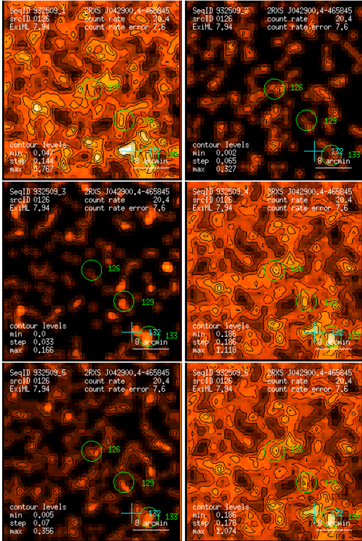
Figure 126: RASS 932509: detection 0126: band rate images, Gaussian filter: (1) PSPC channels 11 – 41, (2) 52 – 90, (3) 91 – 201, (4) 11 – 235, (5) 52 – 201, (6) 11 – 201. Broad band rates in counts/ks. Band rate contour levels in counts/ks/arcmin 2 .
