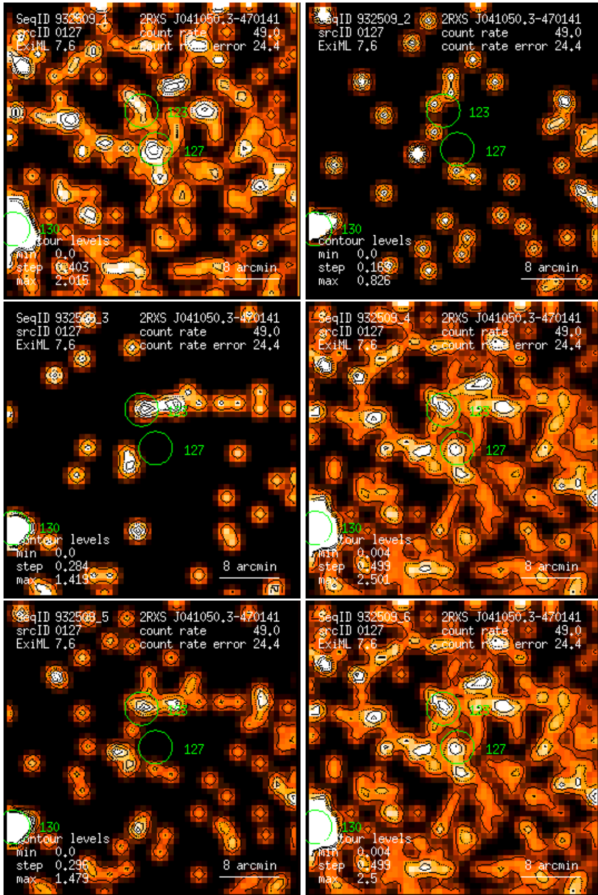
Figure 127: RASS 932509: detection 0127: band rate images, Gaussian filter: (1) PSPC channels 11 – 41, (2) 52 – 90, (3) 91 – 201, (4) 11 – 235, (5) 52 – 201, (6) 11 – 201. Broad band rates in counts/ks. Band rate contour levels in counts/ks/arcmin 2 .
