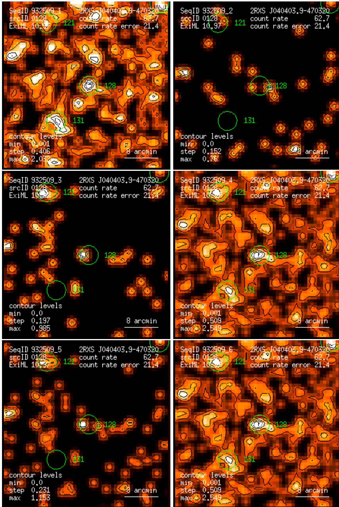
Figure 128: RASS 932509: detection 0128: band rate images, Gaussian filter: (1) PSPC channels 11 – 41, (2) 52 – 90, (3) 91 – 201, (4) 11 – 235, (5) 52 – 201, (6) 11 – 201. Broad band rates in counts/ks. Band rate contour levels in counts/ks/arcmin 2 .
