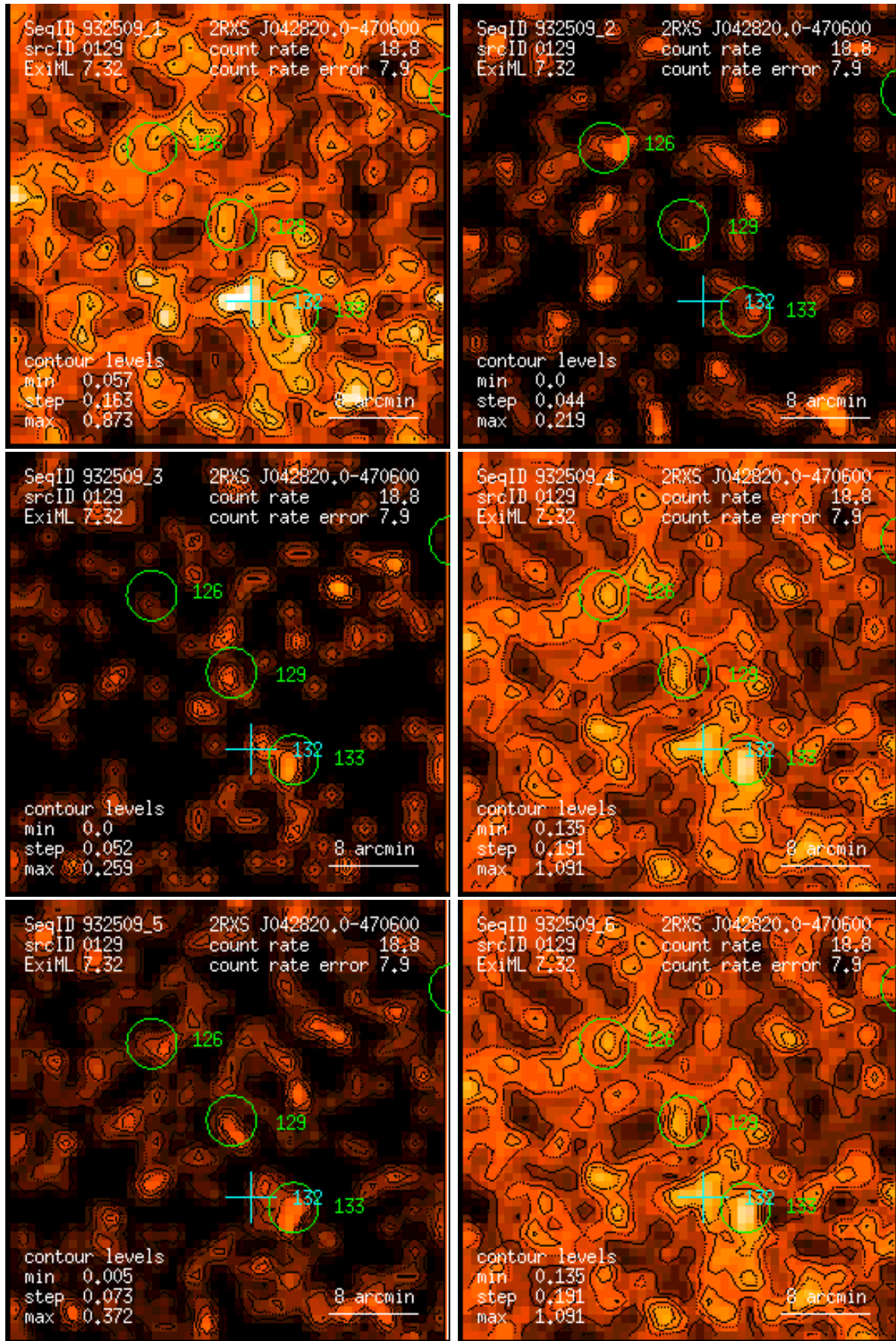
Figure 129: RASS 932509: detection 0129: band rate images, Gaussian filter: (1) PSPC channels 11 – 41, (2) 52 – 90, (3) 91 – 201, (4) 11 – 235, (5) 52 – 201, (6) 11 – 201. Broad band rates in counts/ks. Band rate contour levels in counts/ks/arcmin 2 .
