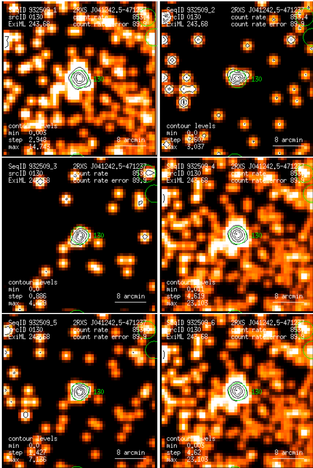
Figure 130: RASS 932509: detection 0130: band rate images, Gaussian filter: (1) PSPC channels 11 – 41, (2) 52 – 90, (3) 91 – 201, (4) 11 – 235, (5) 52 – 201, (6) 11 – 201. Broad band rates in counts/ks. Band rate contour levels in counts/ks/arcmin 2 .
