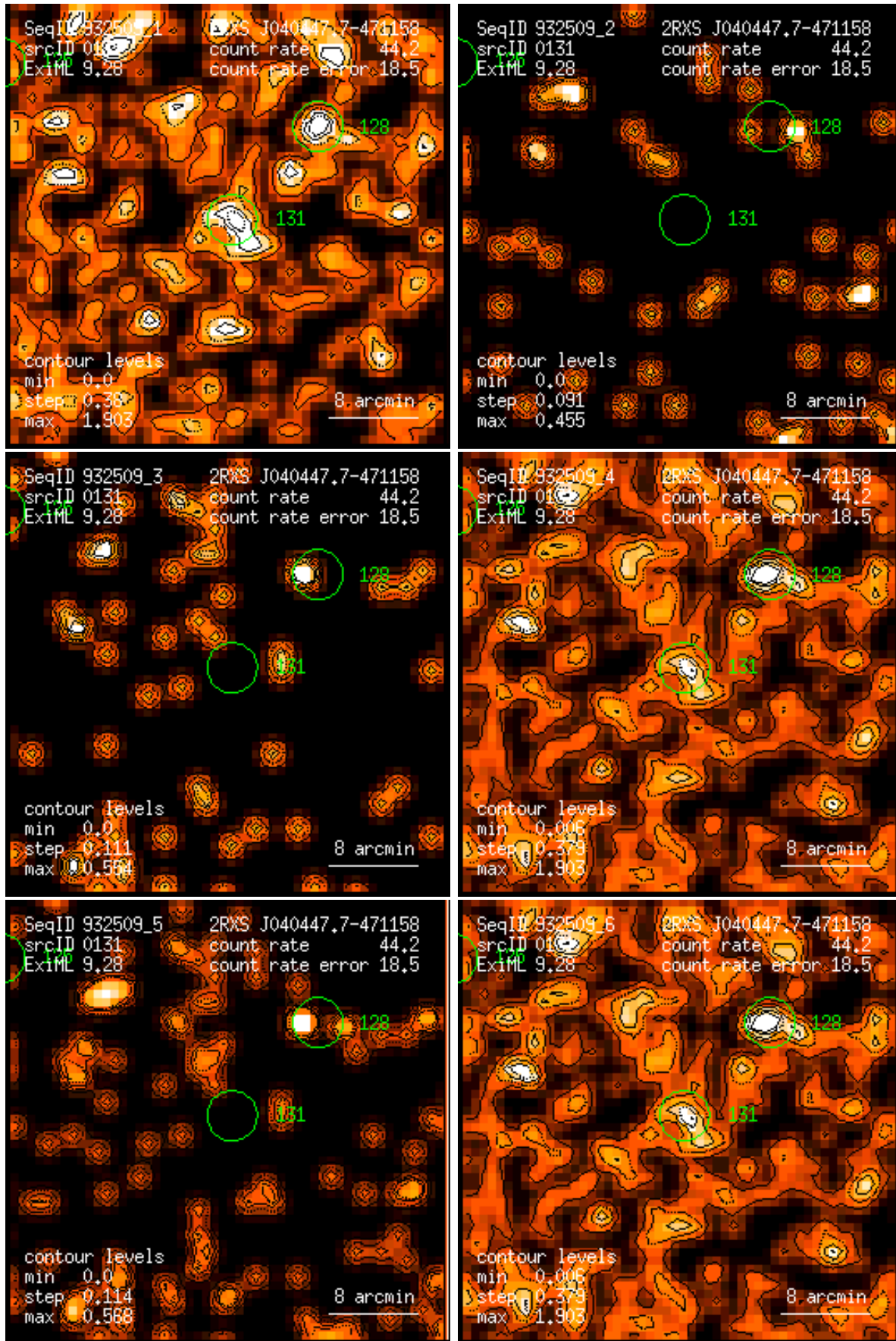
Figure 131: RASS 932509: detection 0131: band rate images, Gaussian filter: (1) PSPC channels 11 – 41, (2) 52 – 90, (3) 91 – 201, (4) 11 – 235, (5) 52 – 201, (6) 11 – 201. Broad band rates in counts/ks. Band rate contour levels in counts/ks/arcmin 2 .
