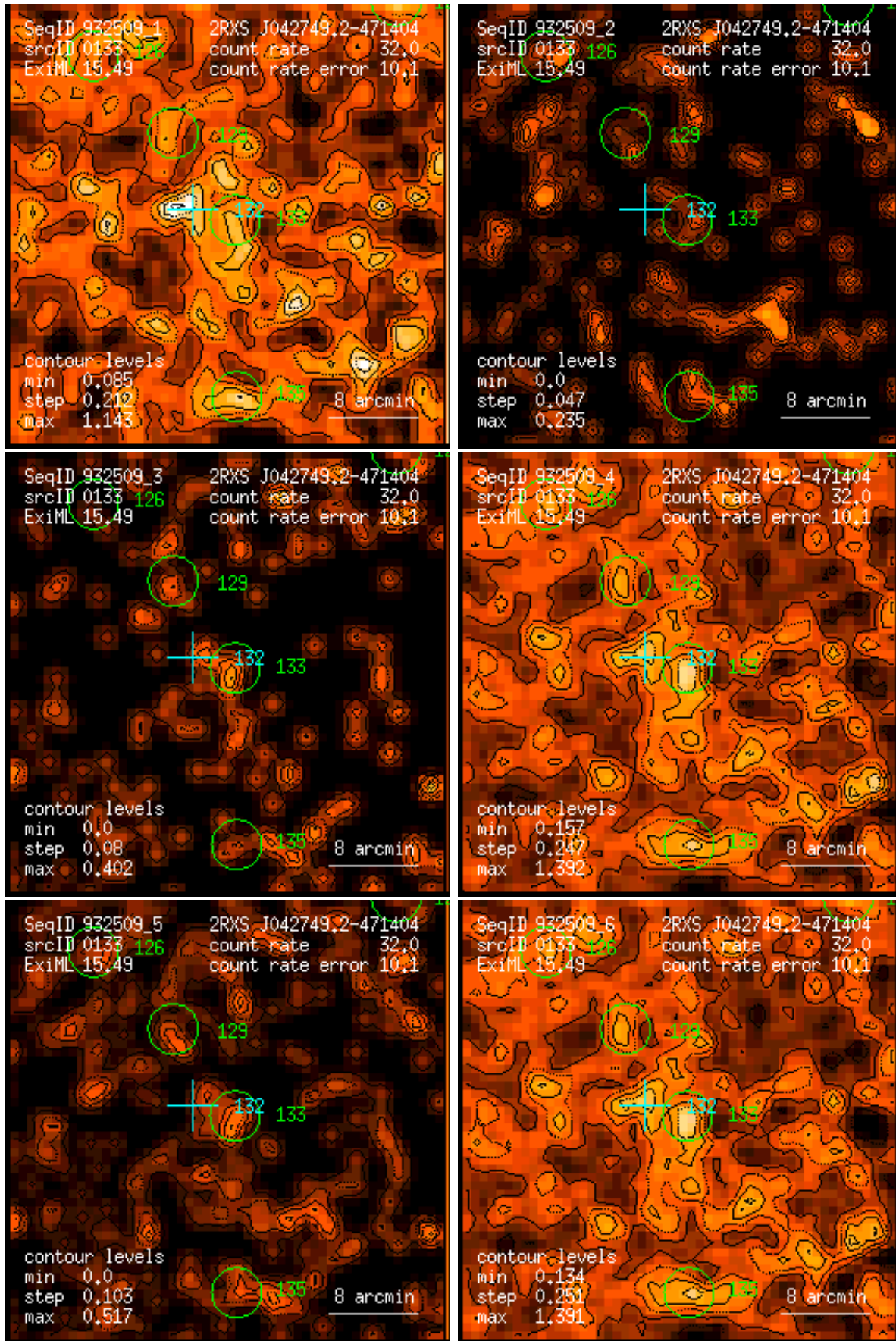
Figure 133: RASS 932509: detection 0133: band rate images, Gaussian filter: (1) PSPC channels 11 – 41, (2) 52 – 90, (3) 91 – 201, (4) 11 – 235, (5) 52 – 201, (6) 11 – 201. Broad band rates in counts/ks. Band rate contour levels in counts/ks/arcmin 2 .
