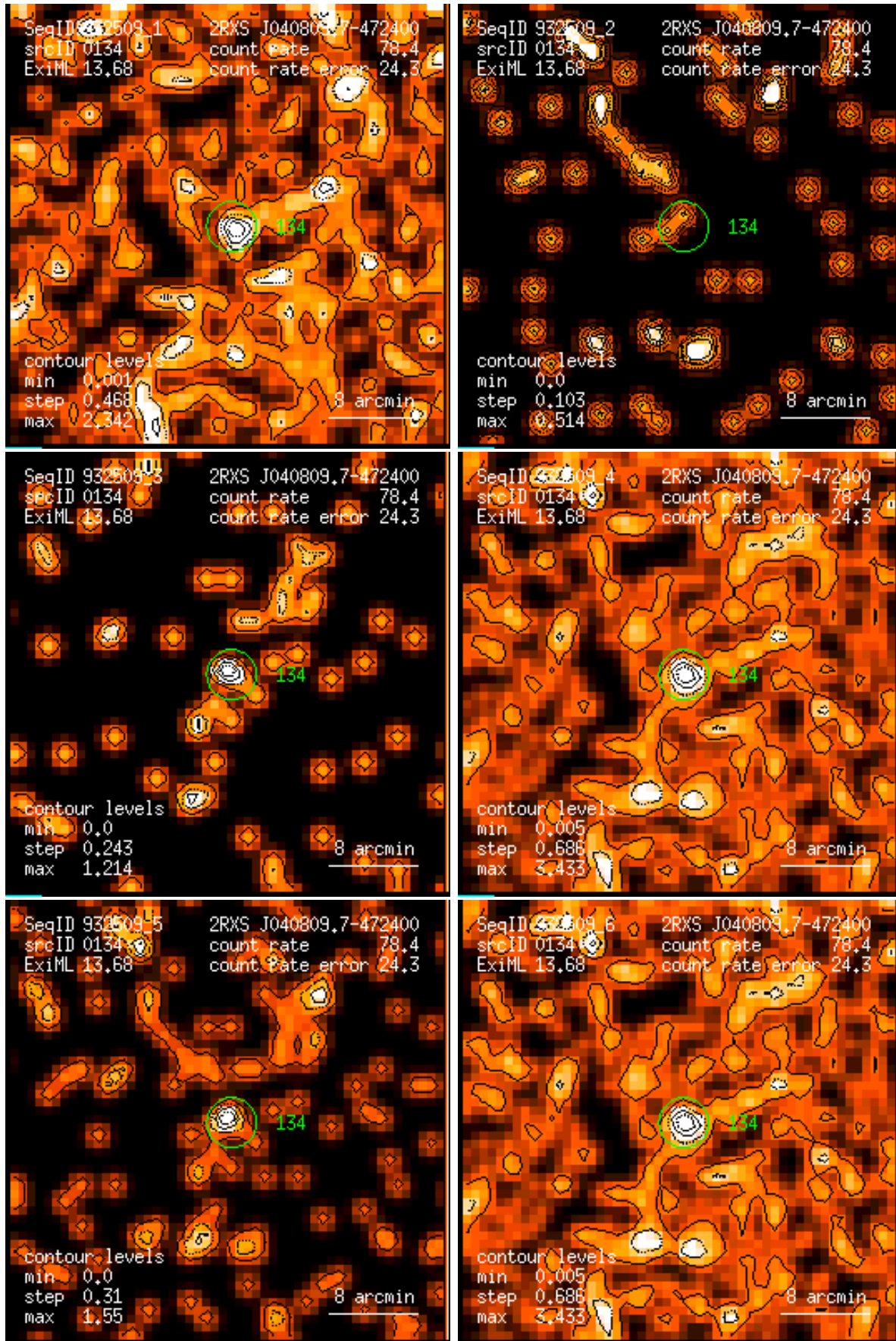
Figure 134: RASS 932509: detection 0134: band rate images, Gaussian filter: (1) PSPC channels 11 – 41, (2) 52 – 90, (3) 91 – 201, (4) 11 – 235, (5) 52 – 201, (6) 11 – 201. Broad band rates in counts/ks. Band rate contour levels in counts/ks/arcmin 2 .
