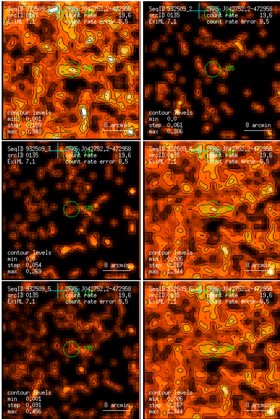
Figure 135: RASS 932509: detection 0135: band rate images, Gaussian filter: (1) PSPC channels 11 – 41, (2) 52 – 90, (3) 91 – 201, (4) 11 – 235, (5) 52 – 201, (6) 11 – 201. Broad band rates in counts/ks. Band rate contour levels in counts/ks/arcmin 2 .
