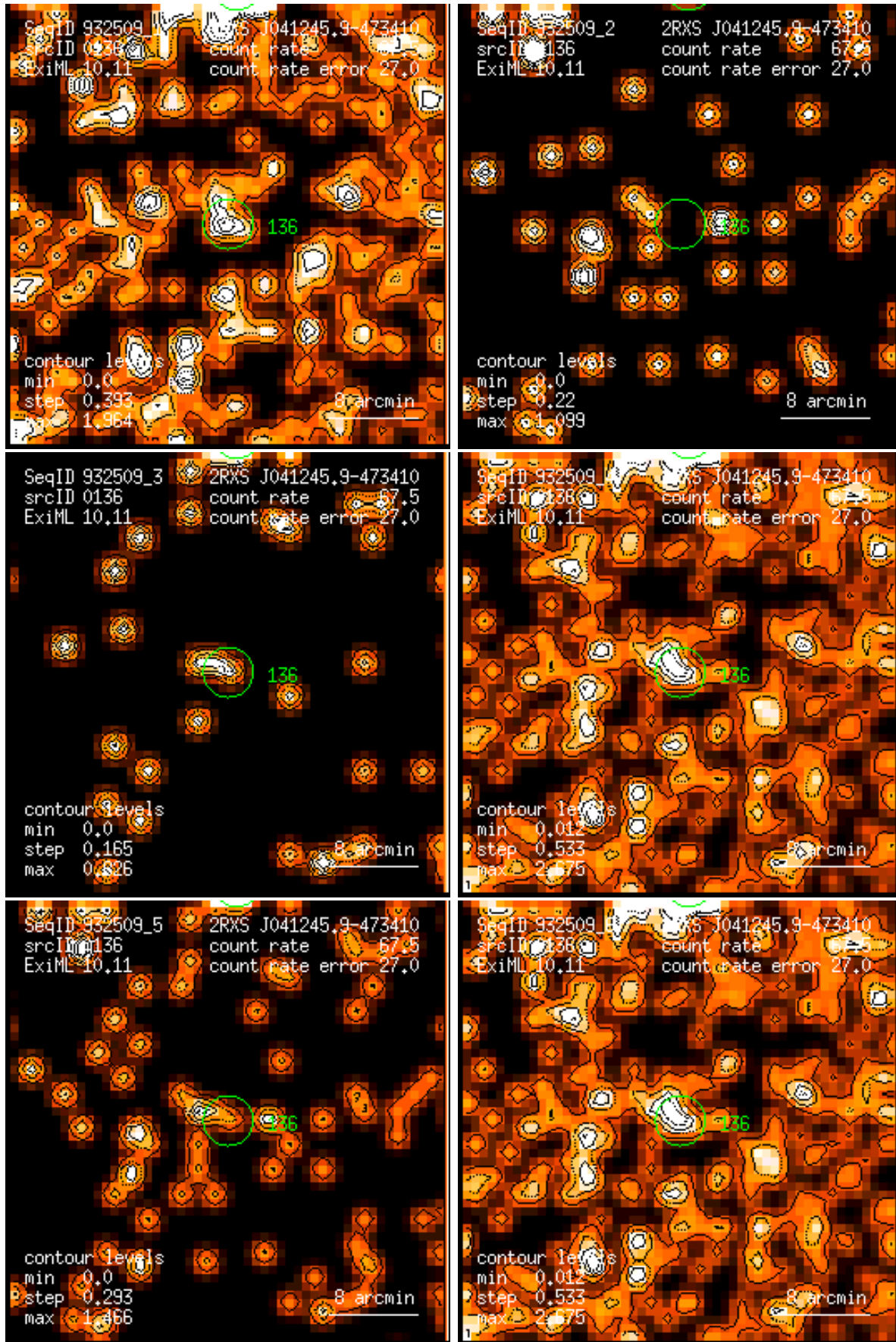
Figure 136: RASS 932509: detection 0136: band rate images, Gaussian filter: (1) PSPC channels 11 – 41, (2) 52 – 90, (3) 91 – 201, (4) 11 – 235, (5) 52 – 201, (6) 11 – 201. Broad band rates in counts/ks. Band rate contour levels in counts/ks/arcmin 2 .
