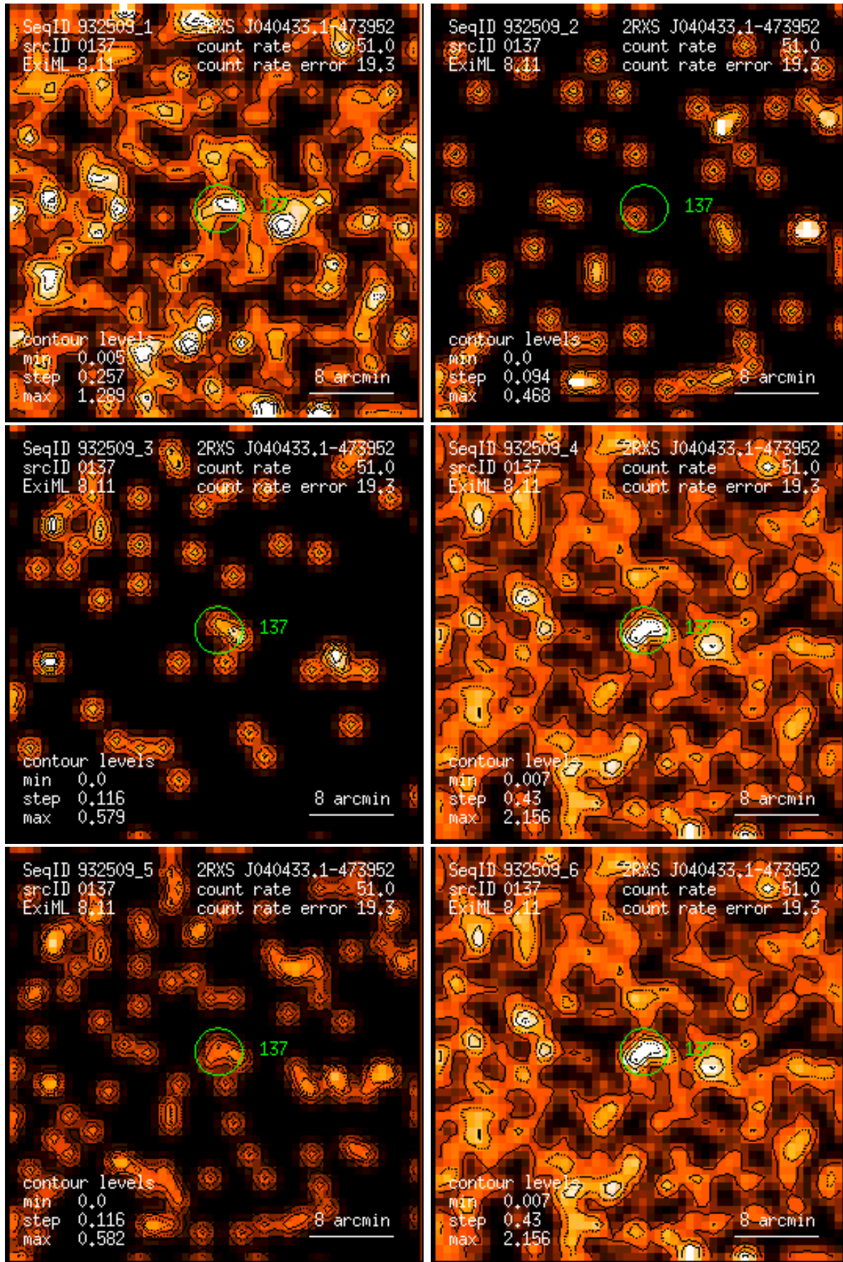
Figure 137: RASS 932509: detection 0137: band rate images, Gaussian filter: (1) PSPC channels 11 – 41, (2) 52 – 90, (3) 91 – 201, (4) 11 – 235, (5) 52 – 201, (6) 11 – 201. Broad band rates in counts/ks. Band rate contour levels in counts/ks/arcmin 2 .
