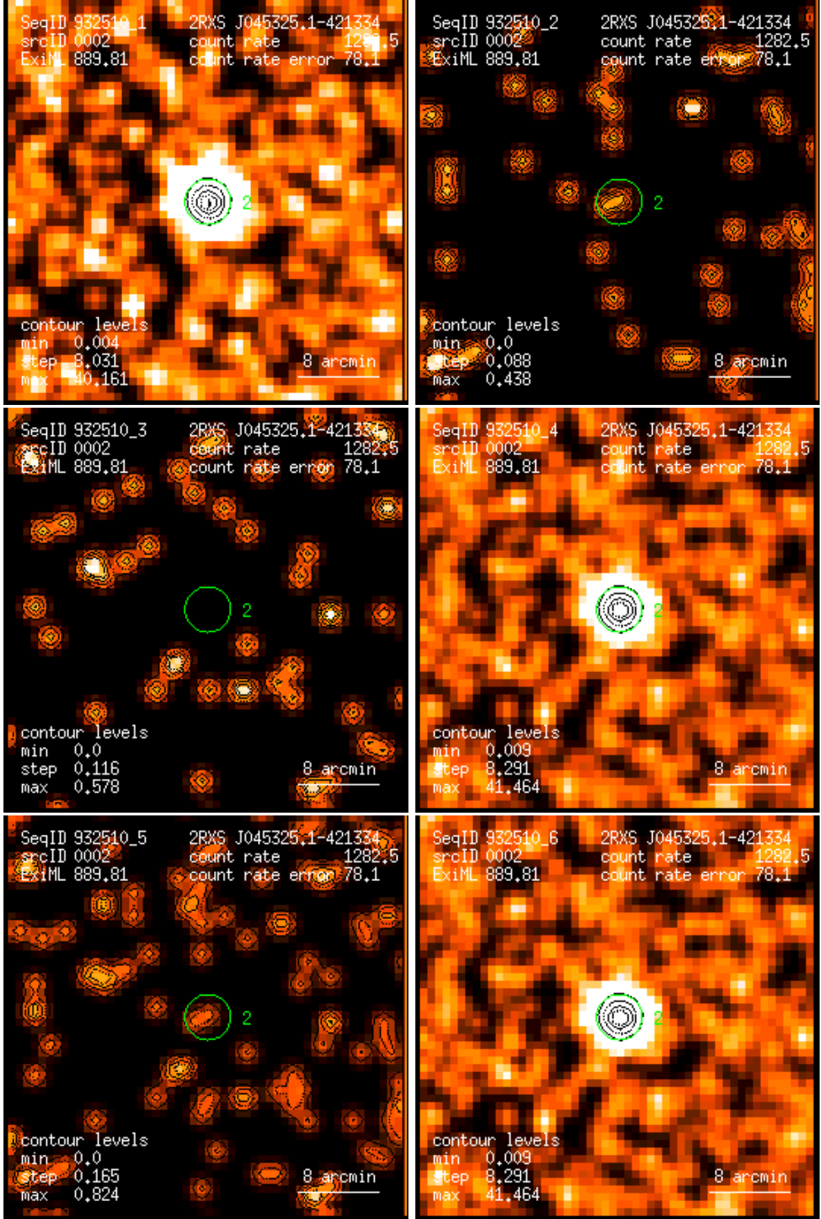
Figure 2: RASS 932510: detection 0002: band rate images, Gaussian filter: (1) PSPC channels 11 – 41, (2) 52 – 90, (3) 91 – 201, (4) 11 – 235, (5) 52 – 201, (6) 11 – 201. Broad band rates in counts/ks. Band rate contour levels in counts/ks/arcmin 2 .
