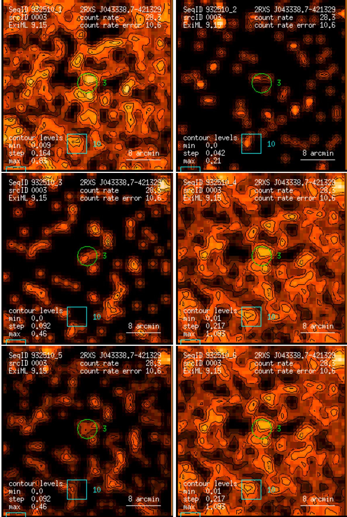
Figure 3: RASS 932510: detection 0003: band rate images, Gaussian filter: (1) PSPC channels 11 – 41, (2) 52 – 90, (3) 91 – 201, (4) 11 – 235, (5) 52 – 201, (6) 11 – 201. Broad band rates in counts/ks. Band rate contour levels in counts/ks/arcmin 2 .
