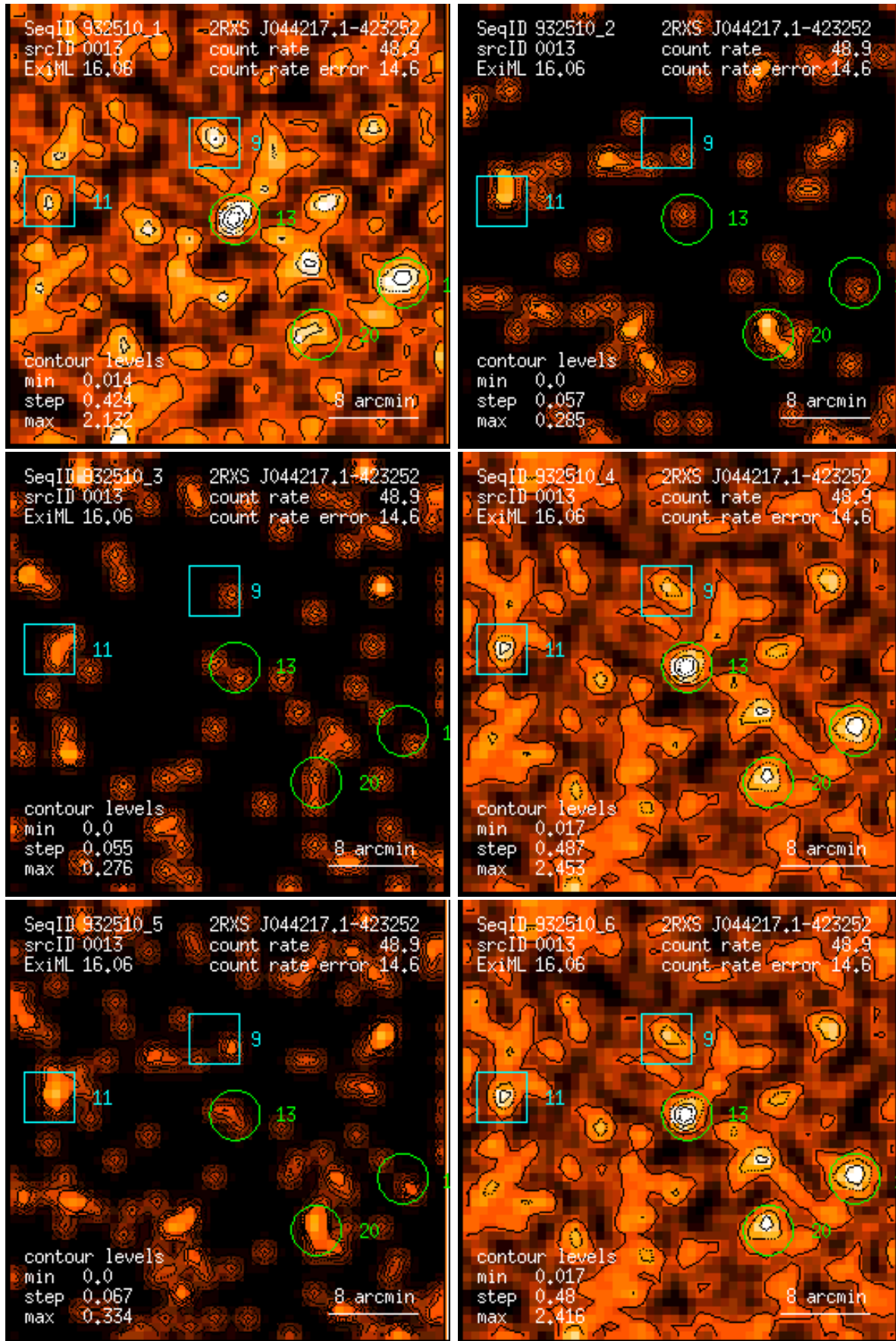
Figure 13: RASS 932510: detection 0013: band rate images, Gaussian filter: (1) PSPC channels 11 – 41, (2) 52 – 90, (3) 91 – 201, (4) 11 – 235, (5) 52 – 201, (6) 11 – 201. Broad band rates in counts/ks. Band rate contour levels in counts/ks/arcmin 2 .
