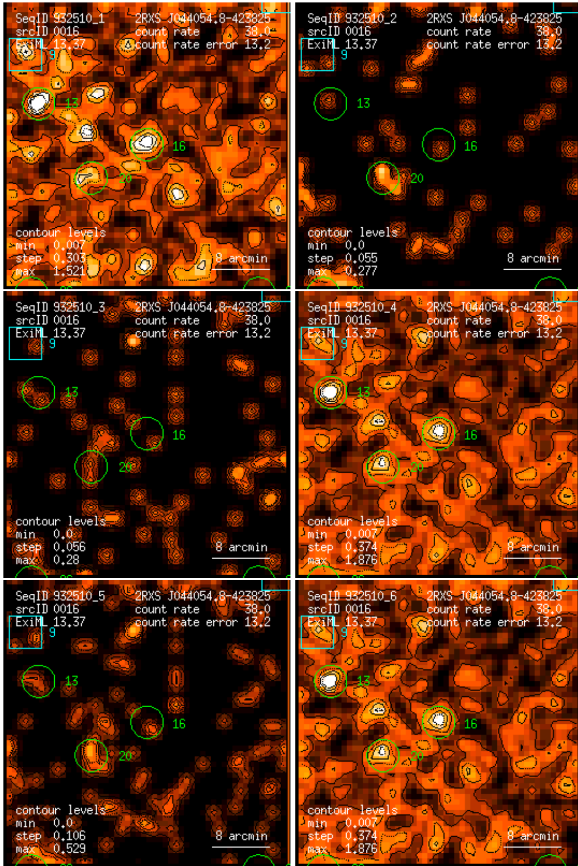
Figure 16: RASS 932510: detection 0016: band rate images, Gaussian filter: (1) PSPC channels 11 – 41, (2) 52 – 90, (3) 91 – 201, (4) 11 – 235, (5) 52 – 201, (6) 11 – 201. Broad band rates in counts/ks. Band rate contour levels in counts/ks/arcmin 2 .
