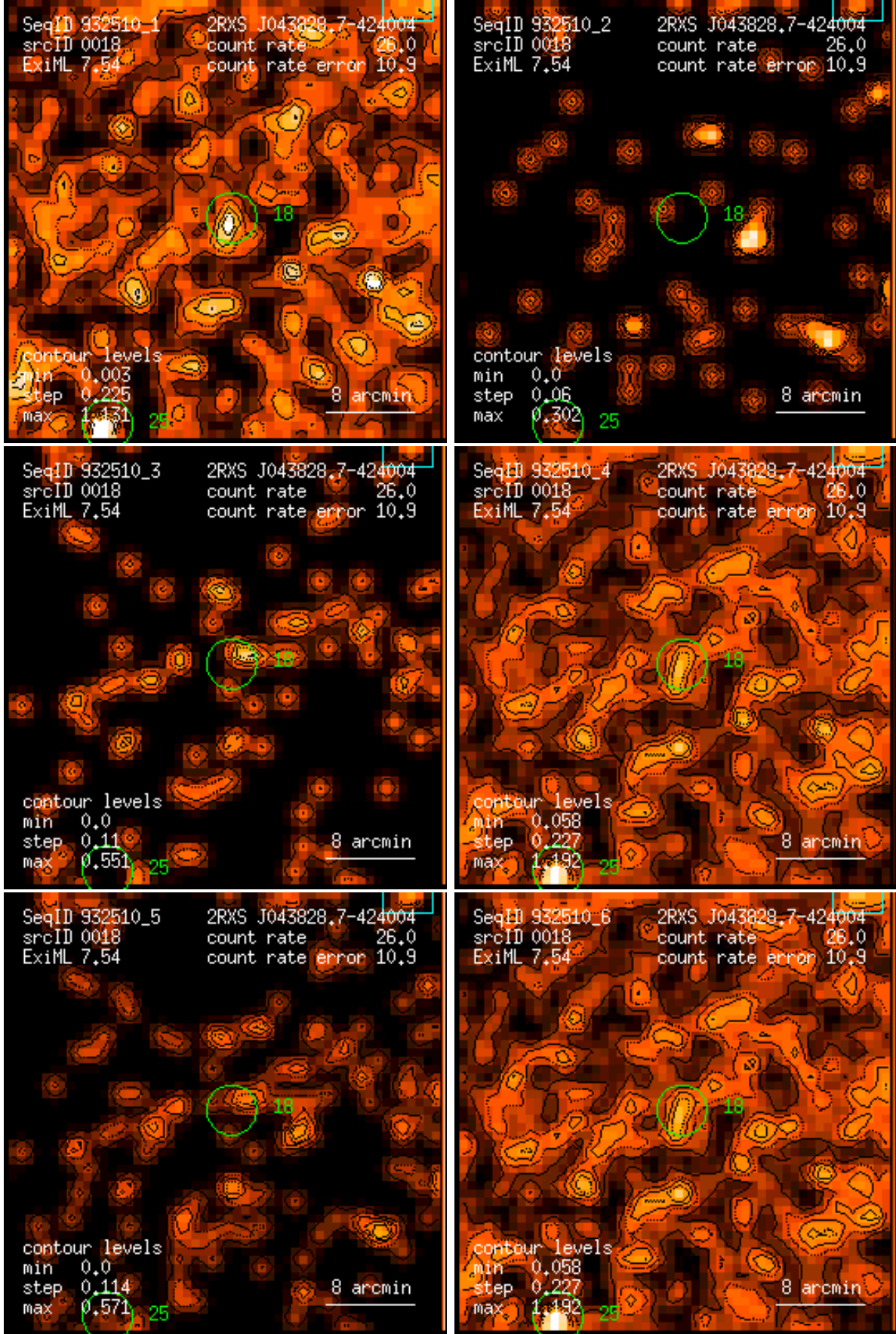
Figure 18: RASS 932510: detection 0018: band rate images, Gaussian filter: (1) PSPC channels 11 – 41, (2) 52 – 90, (3) 91 – 201, (4) 11 – 235, (5) 52 – 201, (6) 11 – 201. Broad band rates in counts/ks. Band rate contour levels in counts/ks/arcmin 2 .
