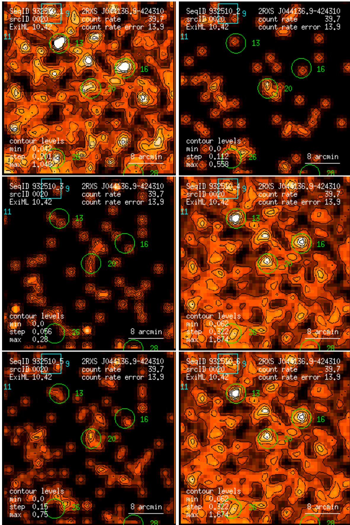
Figure 20: RASS 932510: detection 0020: band rate images, Gaussian filter: (1) PSPC channels 11 – 41, (2) 52 – 90, (3) 91 – 201, (4) 11 – 235, (5) 52 – 201, (6) 11 – 201. Broad band rates in counts/ks. Band rate contour levels in counts/ks/arcmin 2 .
