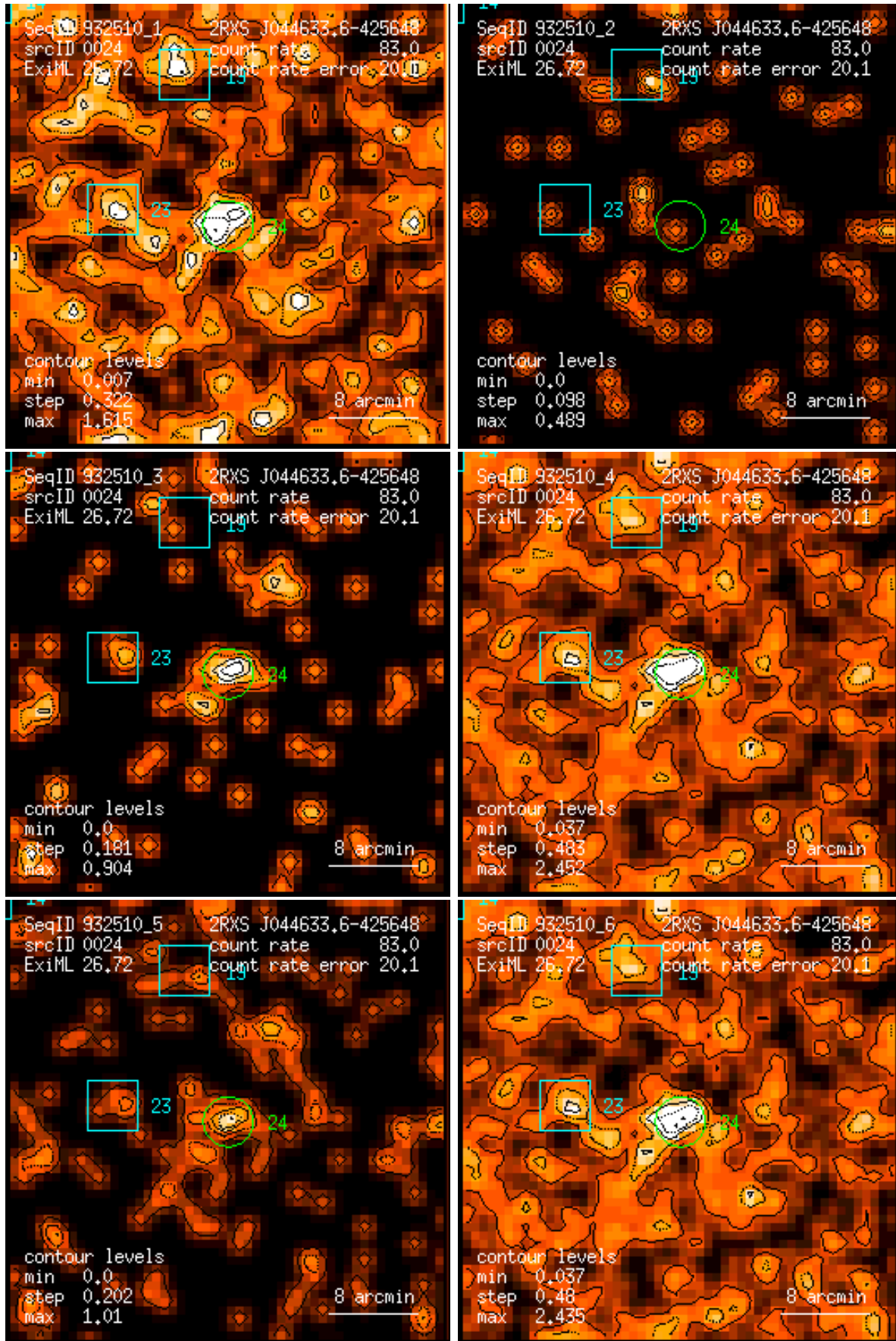
Figure 24: RASS 932510: detection 0024: band rate images, Gaussian filter: (1) PSPC channels 11 – 41, (2) 52 – 90, (3) 91 – 201, (4) 11 – 235, (5) 52 – 201, (6) 11 – 201. Broad band rates in counts/ks. Band rate contour levels in counts/ks/arcmin 2 .
