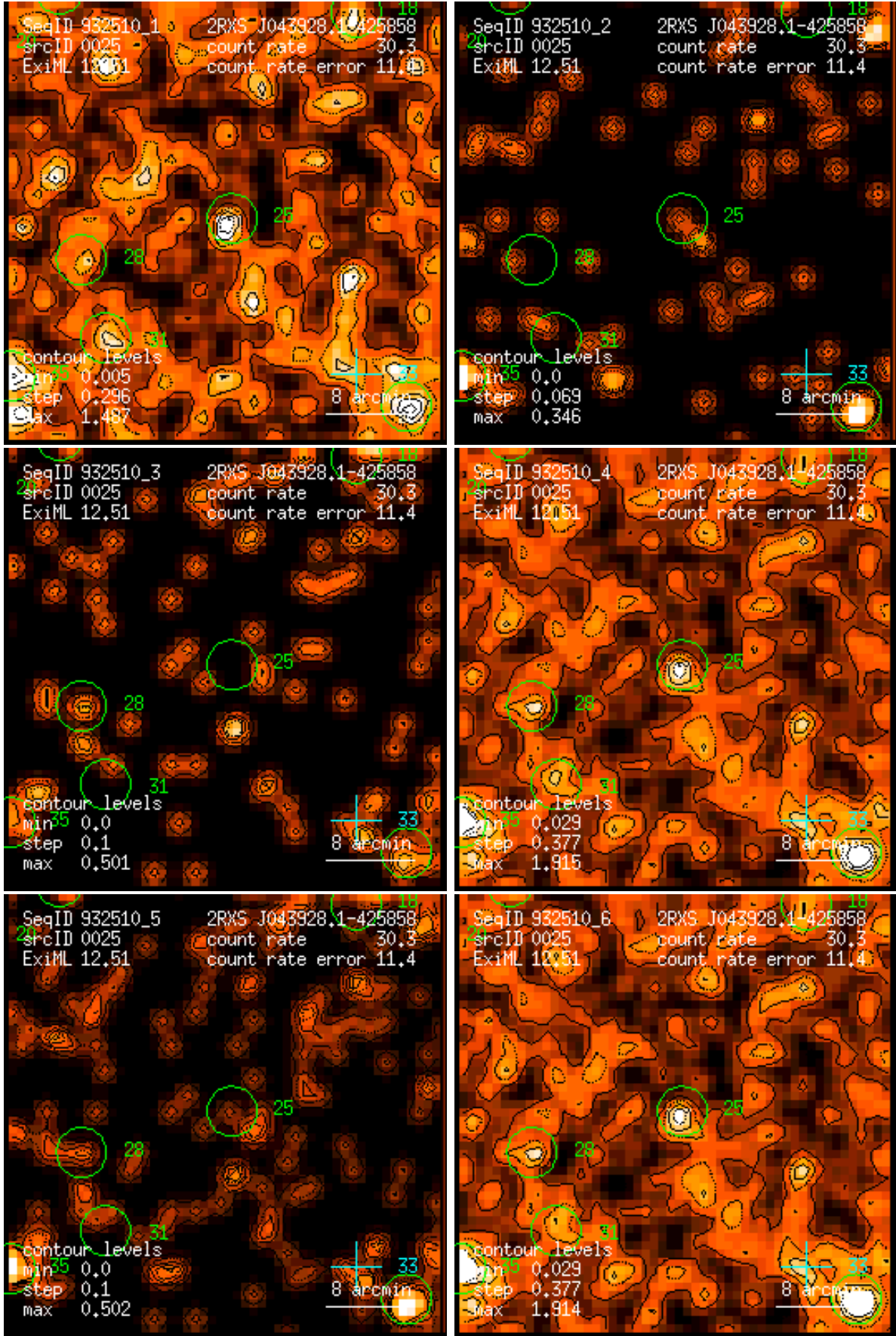
Figure 25: RASS 932510: detection 0025: band rate images, Gaussian filter: (1) PSPC channels 11 – 41, (2) 52 – 90, (3) 91 – 201, (4) 11 – 235, (5) 52 – 201, (6) 11 – 201. Broad band rates in counts/ks. Band rate contour levels in counts/ks/arcmin 2 .
