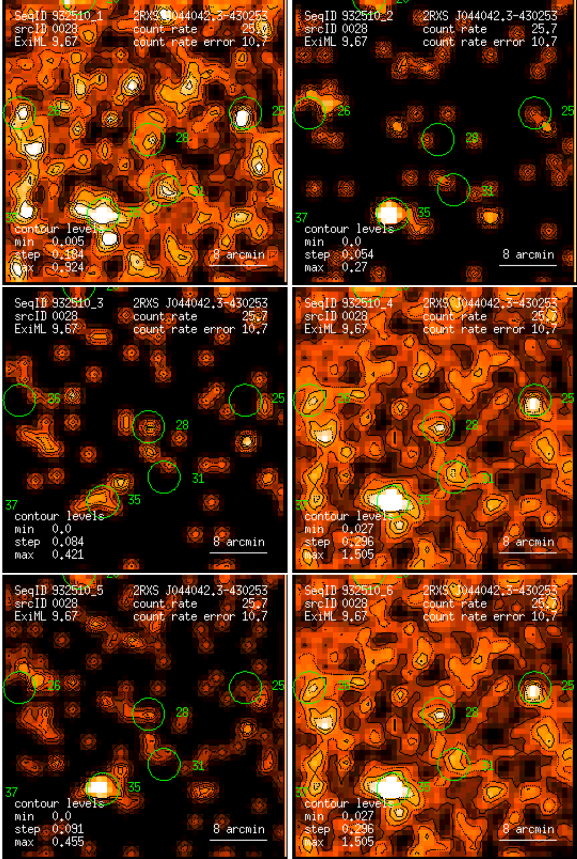
Figure 28: RASS 932510: detection 0028: band rate images, Gaussian filter: (1) PSPC channels 11 – 41, (2) 52 – 90, (3) 91 – 201, (4) 11 – 235, (5) 52 – 201, (6) 11 – 201. Broad band rates in counts/ks. Band rate contour levels in counts/ks/arcmin 2 .
