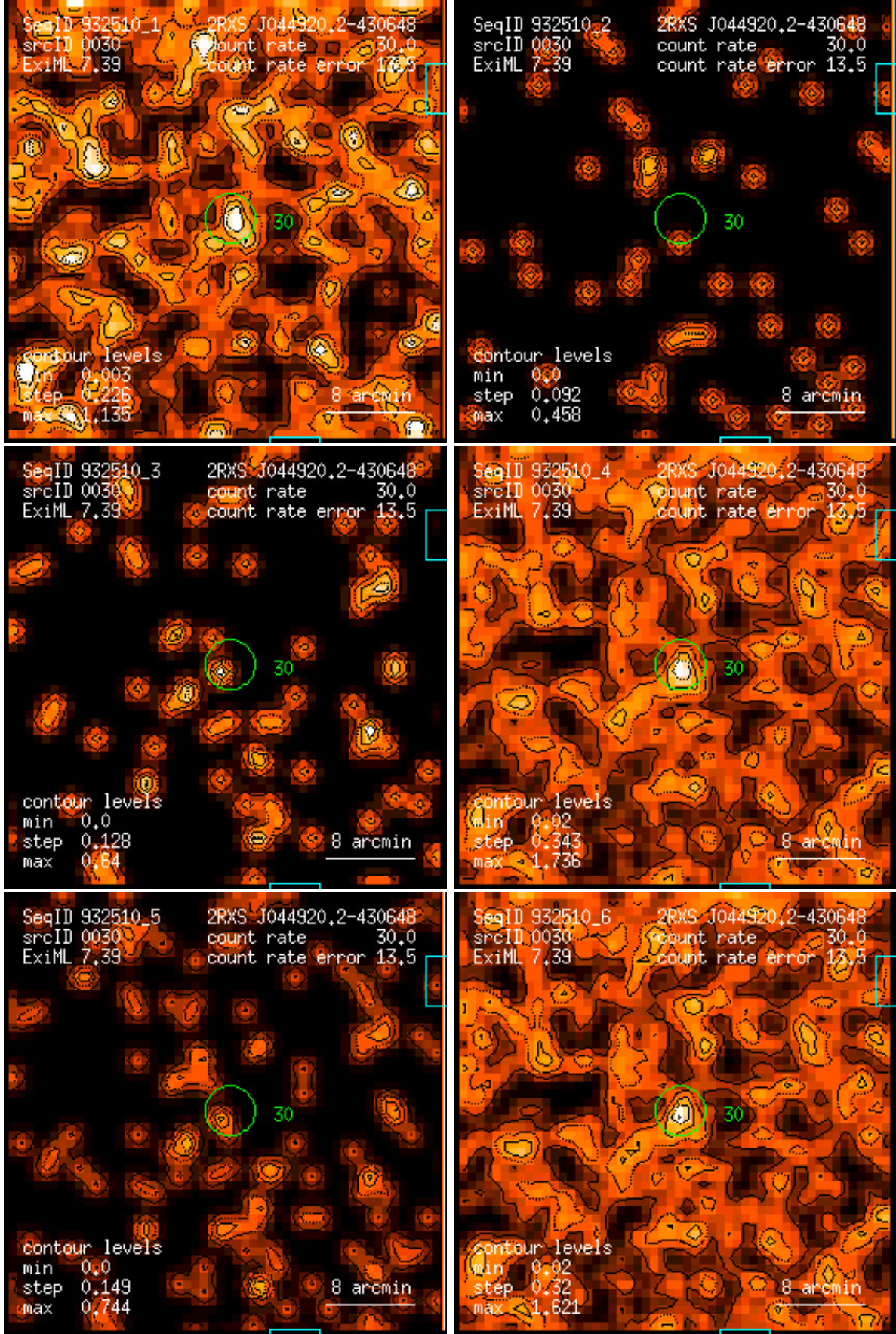
Figure 30: RASS 932510: detection 0030: band rate images, Gaussian filter: (1) PSPC channels 11 – 41, (2) 52 – 90, (3) 91 – 201, (4) 11 – 235, (5) 52 – 201, (6) 11 – 201. Broad band rates in counts/ks. Band rate contour levels in counts/ks/arcmin 2 .
