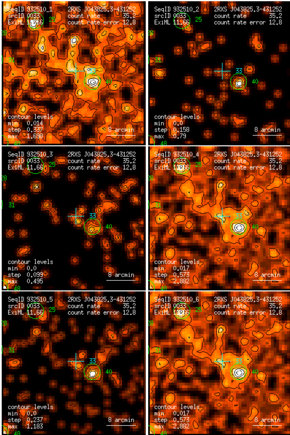
Figure 33: RASS 932510: detection 0033: band rate images, Gaussian filter: (1) PSPC channels 11 – 41, (2) 52 – 90, (3) 91 – 201, (4) 11 – 235, (5) 52 – 201, (6) 11 – 201. Broad band rates in counts/ks. Band rate contour levels in counts/ks/arcmin 2 .
