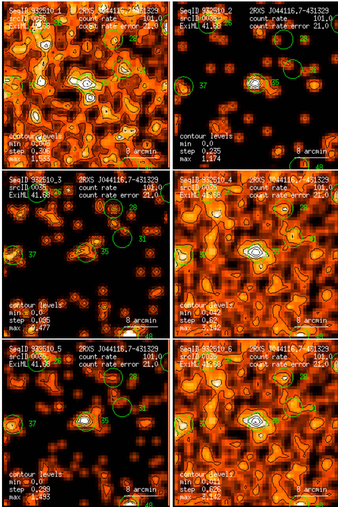
Figure 35: RASS 932510: detection 0035: band rate images, Gaussian filter: (1) PSPC channels 11 – 41, (2) 52 – 90, (3) 91 – 201, (4) 11 – 235, (5) 52 – 201, (6) 11 – 201. Broad band rates in counts/ks. Band rate contour levels in counts/ks/arcmin 2 .
