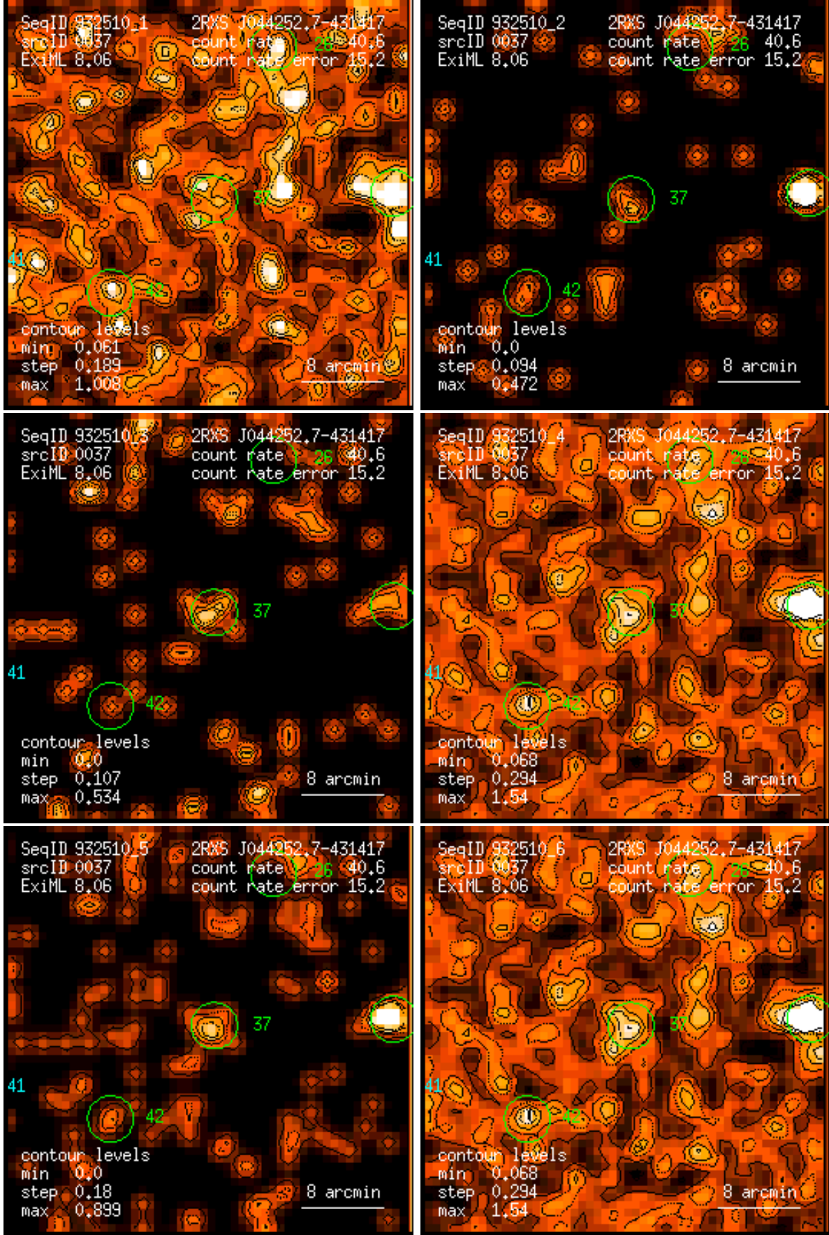
Figure 37: RASS 932510: detection 0037: band rate images, Gaussian filter: (1) PSPC channels 11 – 41, (2) 52 – 90, (3) 91 – 201, (4) 11 – 235, (5) 52 – 201, (6) 11 – 201. Broad band rates in counts/ks. Band rate contour levels in counts/ks/arcmin 2 .
